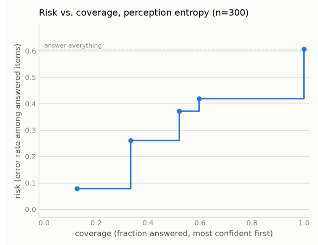
Figure 1. Risk-coverage for perception entropy, Qwen2.5-VL-3B, n = 300 . Deferring the highest-entropy items first traces AURC 0.410 against a 0.607 random-deferral baseline. The curve is the practitioner-facing form of the result: at a 10% risk target the rule retains 21.3% coverage, and token log-probability cannot hold error below 40% at any coverage.
