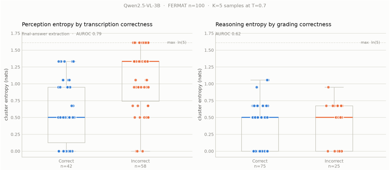
Figure 2: Final result for both arms, n = 100 . Left: perception entropy by transcription correctness (AUROC 0.788, 95% CI [0.697, 0.869]). Right: reasoning entropy by grading correctness at K = 5 (AUROC 0.618, 95% CI [0.489, 0.741] – includes chance).
