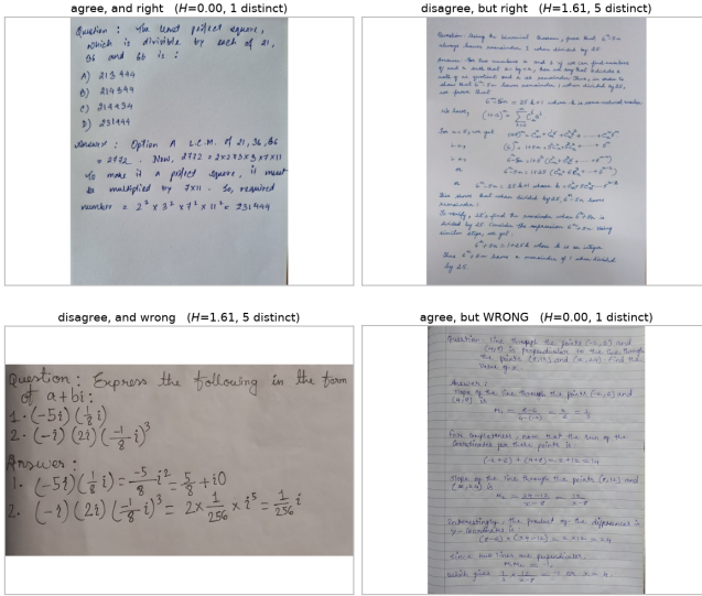
Figure 2: The four quadrants of entropy \times correctness, on real pages, Qwen2.5-VL-3B. Top left is the signal working: five identical transcriptions, correct. Bottom left is it working in the other direction. Top right is a false alarm — the samples disagree but the majority is still right, the cost of any deferral rule. Bottom right is the bound on the method: five identical transcriptions, all wrong. That quadrant is invisible to self-disagreement by construction, and it is where the audit of §6 finds the unearned passes concentrate.
