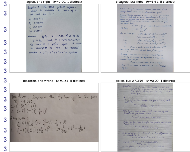
Figure 2. The four quadrants of entropy \times correctness, on real pages, Qwen2.5-VL-3B. Top left is the signal working: five identical transcriptions, correct. Bottom left is it working in the other direction. Top right is a false alarm, in which the samples disagree while the majority remains correct, which is the cost of any deferral rule. Bottom right is the bound on the method: five identical transcriptions, all wrong. That quadrant is invisible to self-disagreement by construction, and it is where the audit of §6 finds the unearned passes concentrate.
