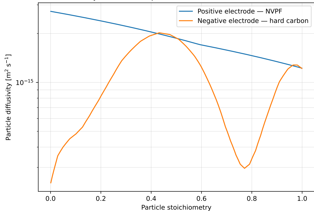
Chayambuka2022 particle diffusivities at 298.15 K
