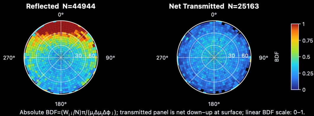
MC with 100K photons, Case 4.
