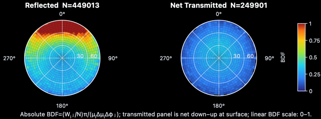
MC with 1M photons, Case 4.
