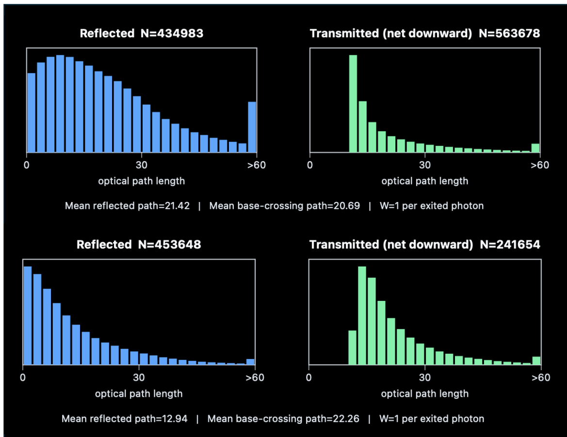
MC path length histograms with 1M photons. Case 1 (top row) and Case 4 (bottom).
