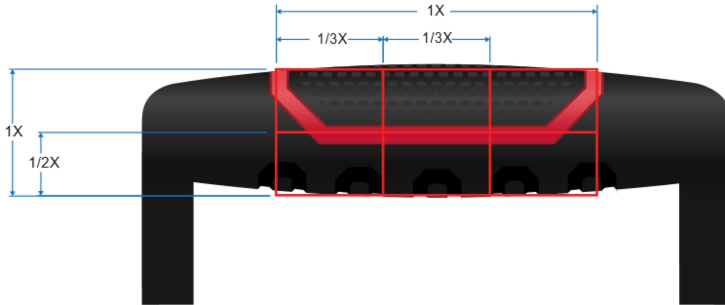
Proportion Grid for Symmetrical Handle
