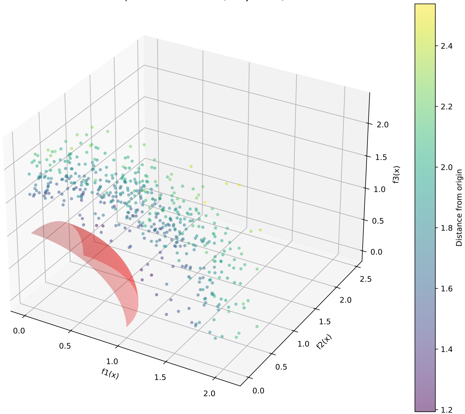
DTLZ2: Spherical Pareto Front (3 objectives)
