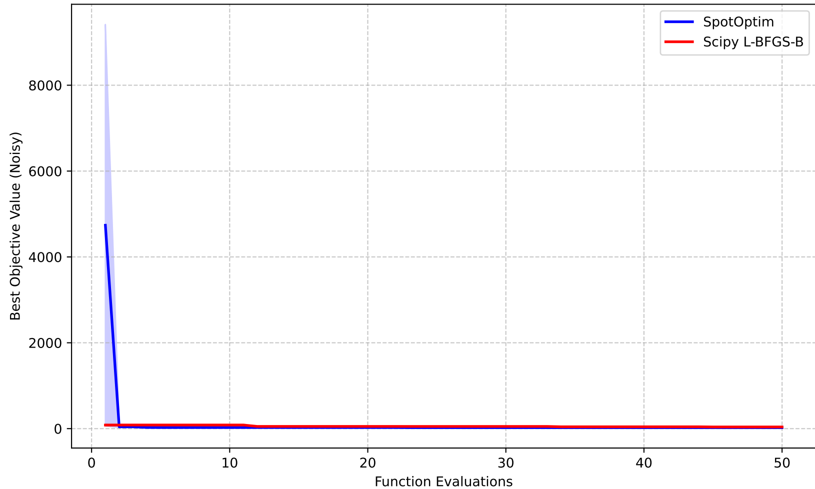
Optimization Progress Comparison (Noisy)
