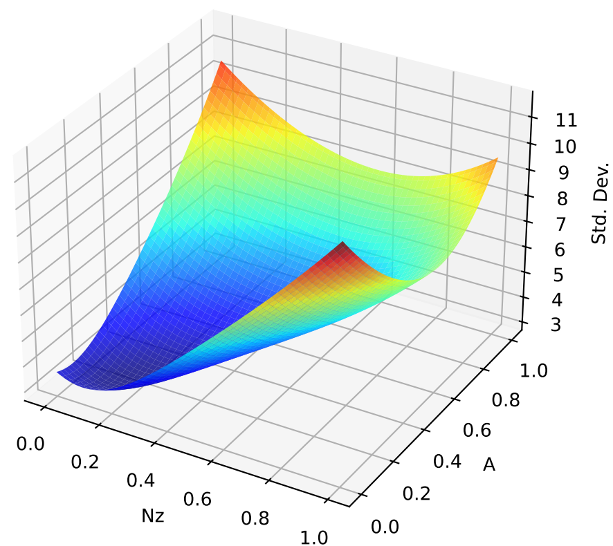
Uncertainty Contour
