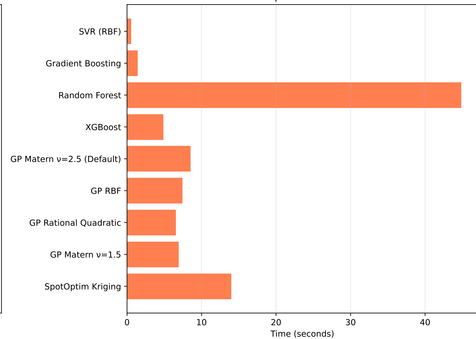
Optimization Efficiency
