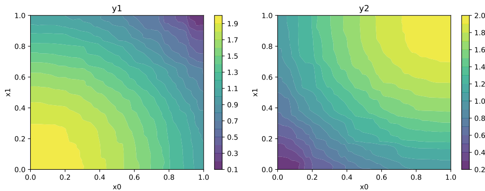
Figure 60.2.: Contours of the two objectives of the mo_conv2_max function
