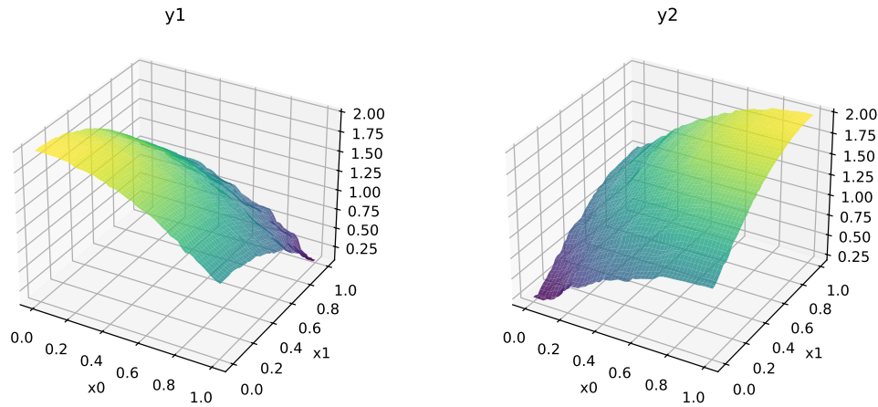
Figure 60.1.: Surfaces of the two objectives of the mo_conv2_max function
