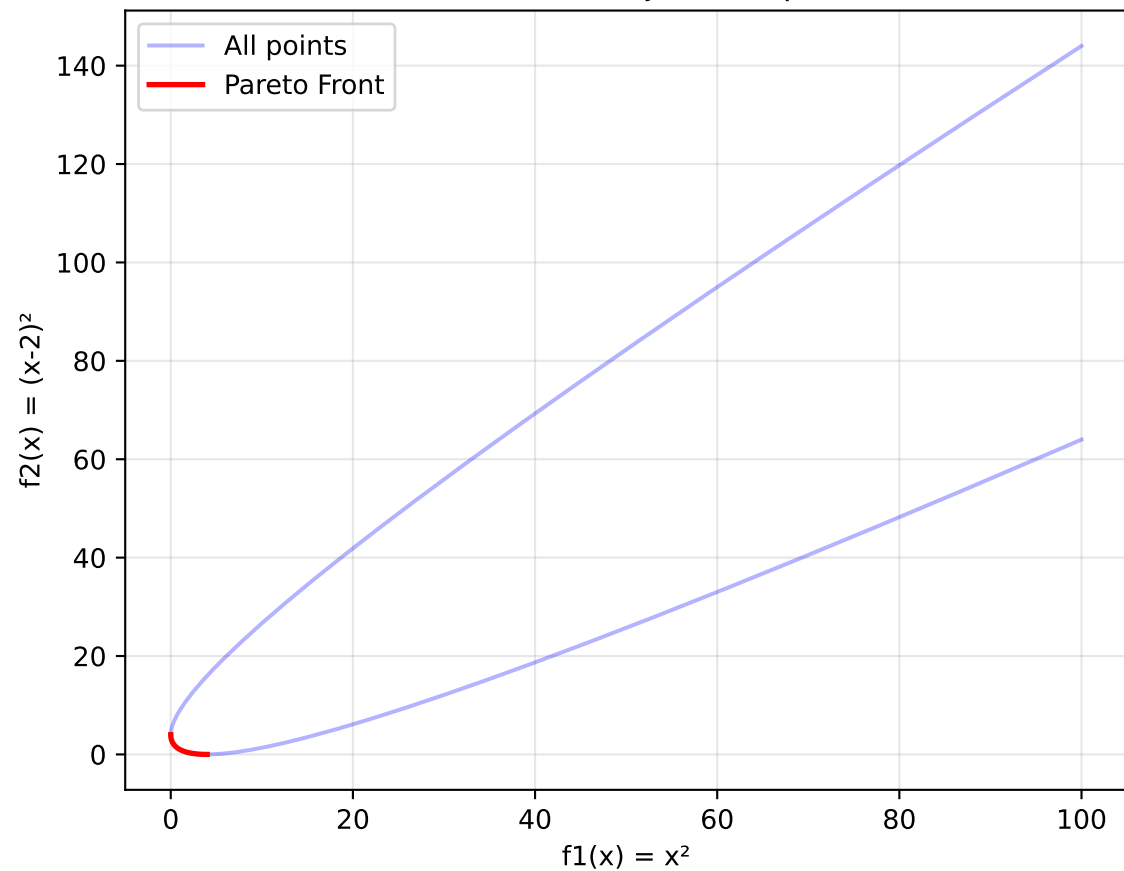
Schaffer N1: Objective Space
