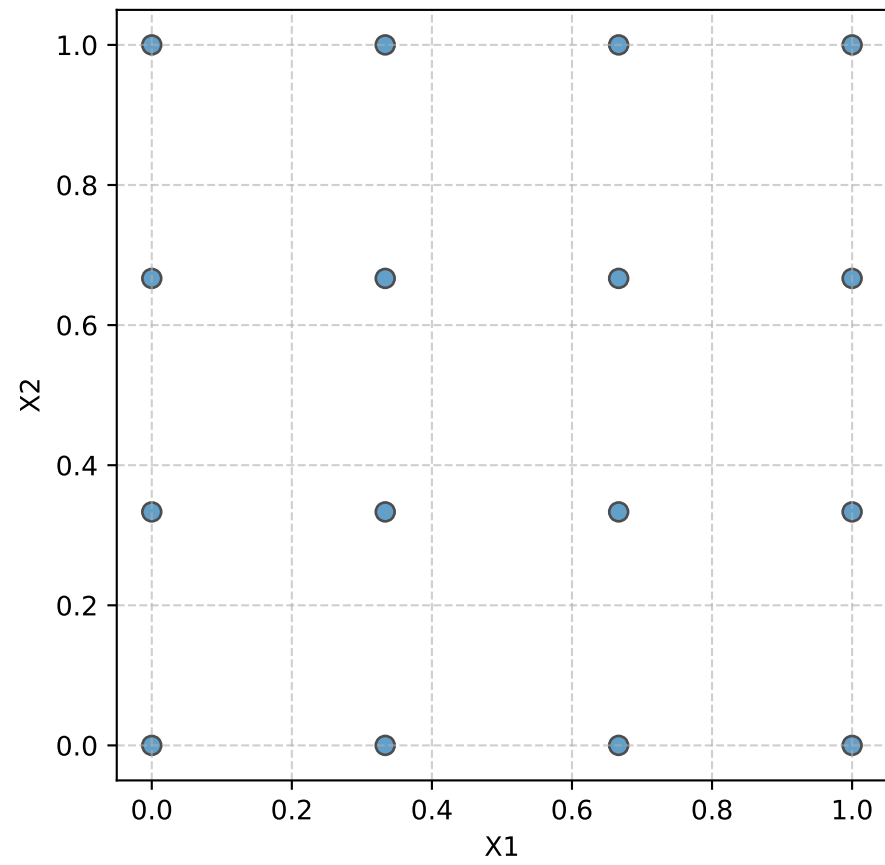
Sobol mmphi = 28.467
