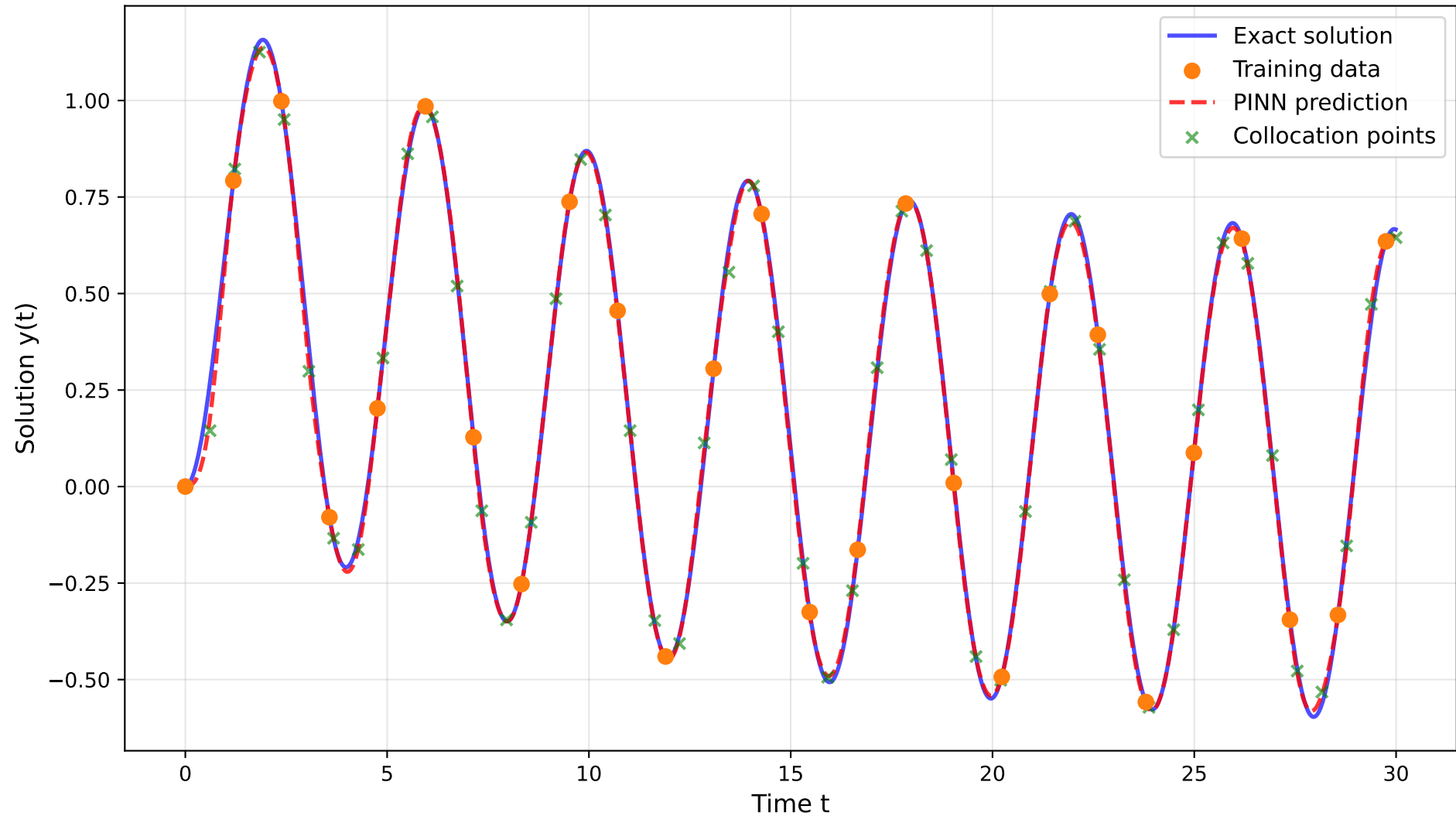
PINN Solution at Epoch 30000
