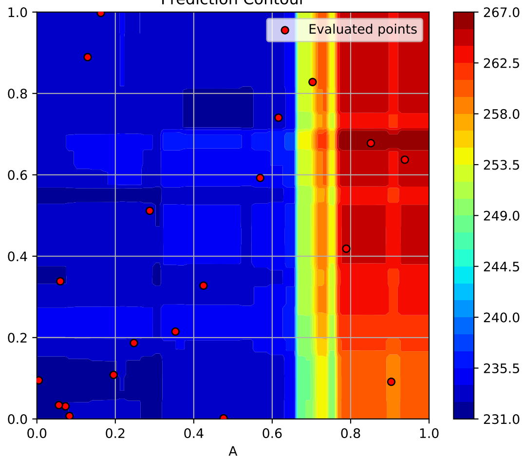
Prediction Contour
