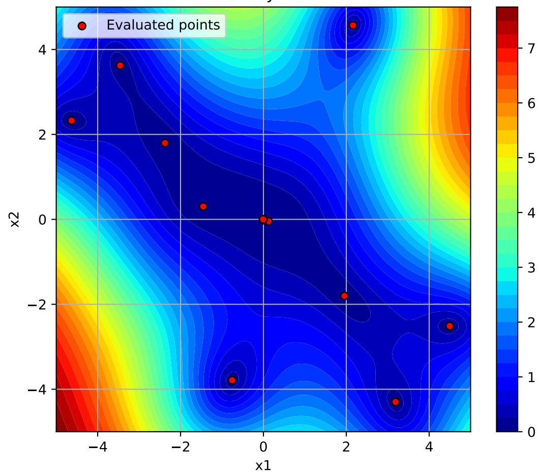
Uncertainty Contour
