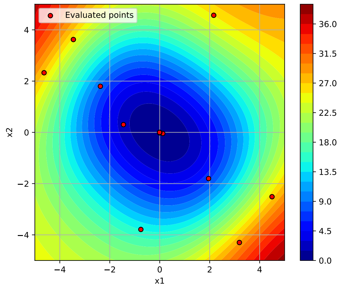
Prediction Contour
