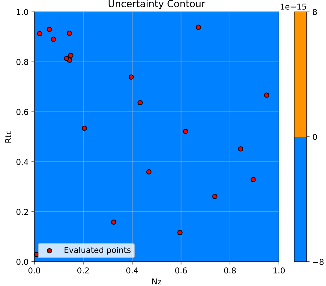
Uncertainty Contour
