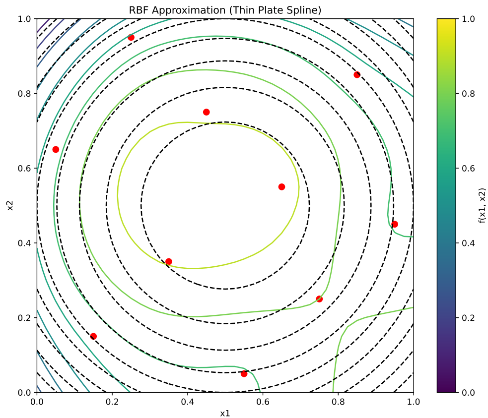
Figure 76.3.: RBF Approximation.
