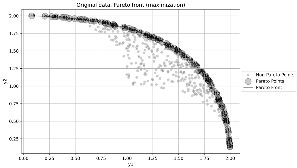
Figure 29.3.: Pareto front of the original data
