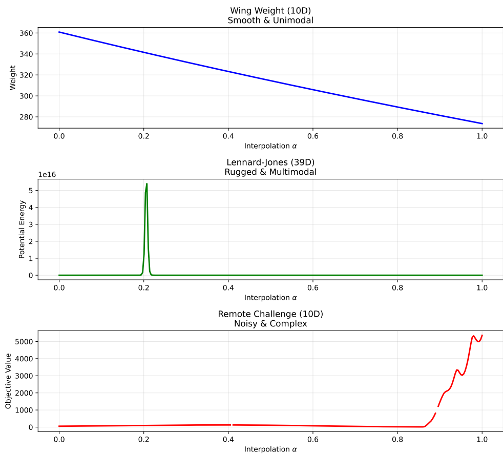
Figure 80.1.: 1D Slice through High-Dimensional Landscapes
