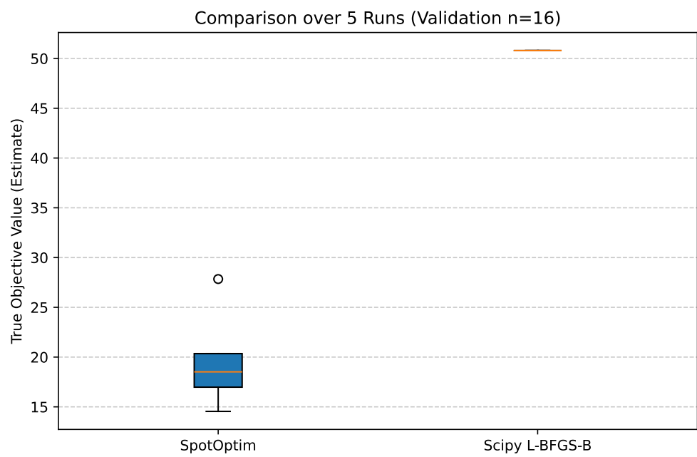
Figure 80.3.: Comparison of Validated True Means (Lower is Better)
