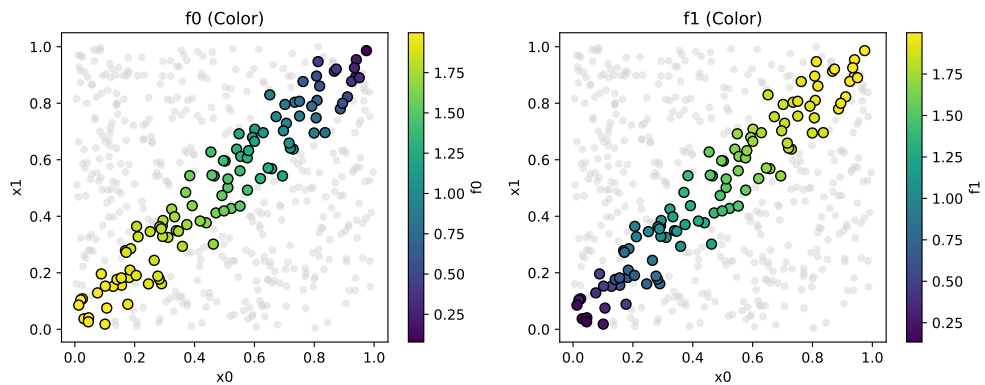
Figure 29.4.: Pareto-optimal points in the input space
