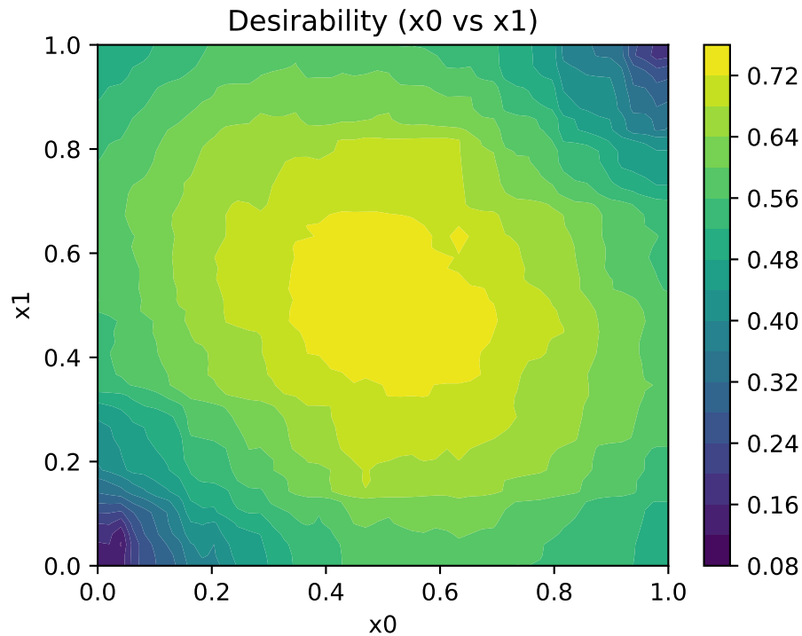
Figure 29.5.: Desirability function for multi-objective optimization
