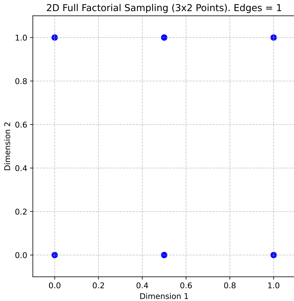
Figure 72.4.: 2D Full Factorial Sampling (3x2 Points). Edges = 1
