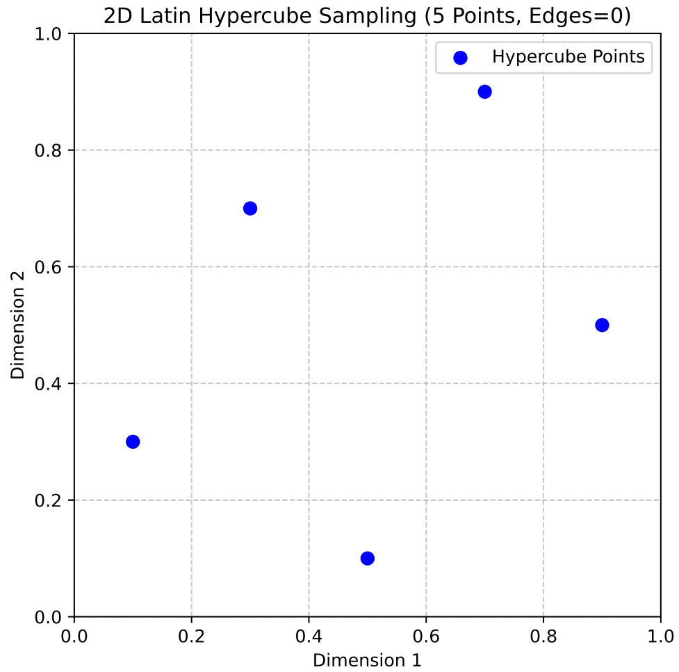
Figure 72.5.: 2D Latin Hypercube Sampling (5 Points, Edges=0)
