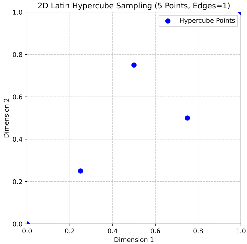
Figure 72.6.: 2D Latin Hypercube Sampling (5 Points, Edges=1)
