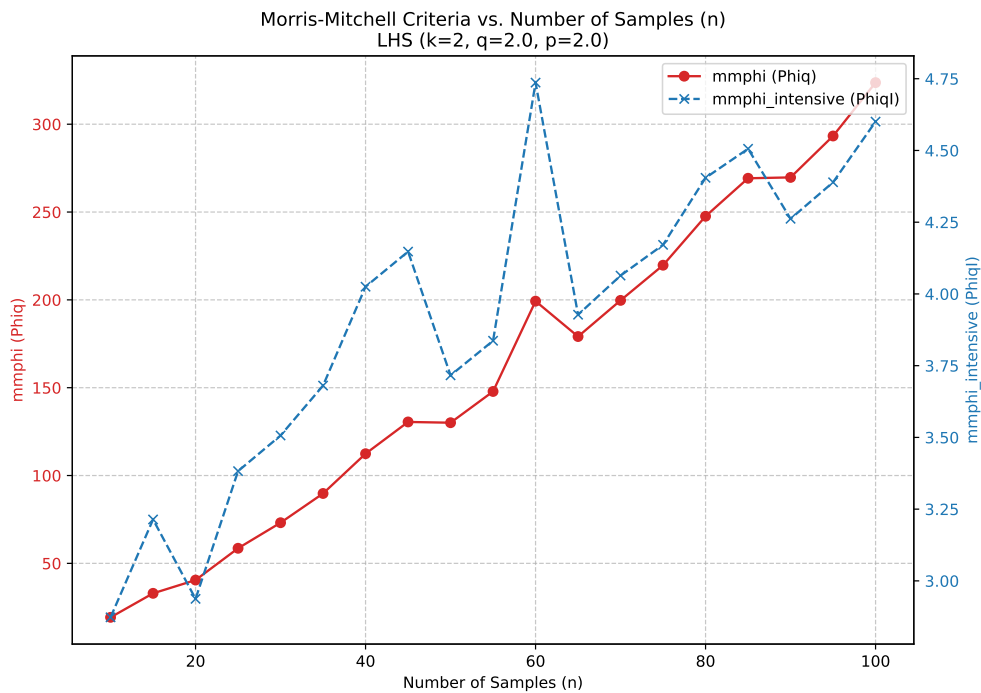
Figure 72.11.: Comparison of the two Morris-Mitchell Criteria for Different Sample Sizes
