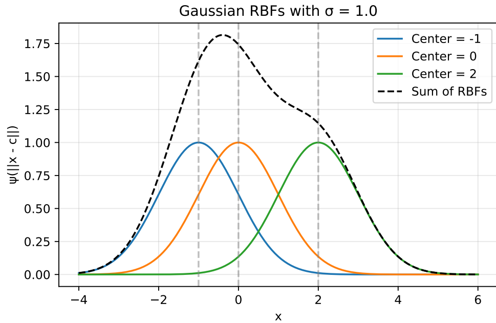
Figure 76.2.: Sum of Gaussian RBFs
