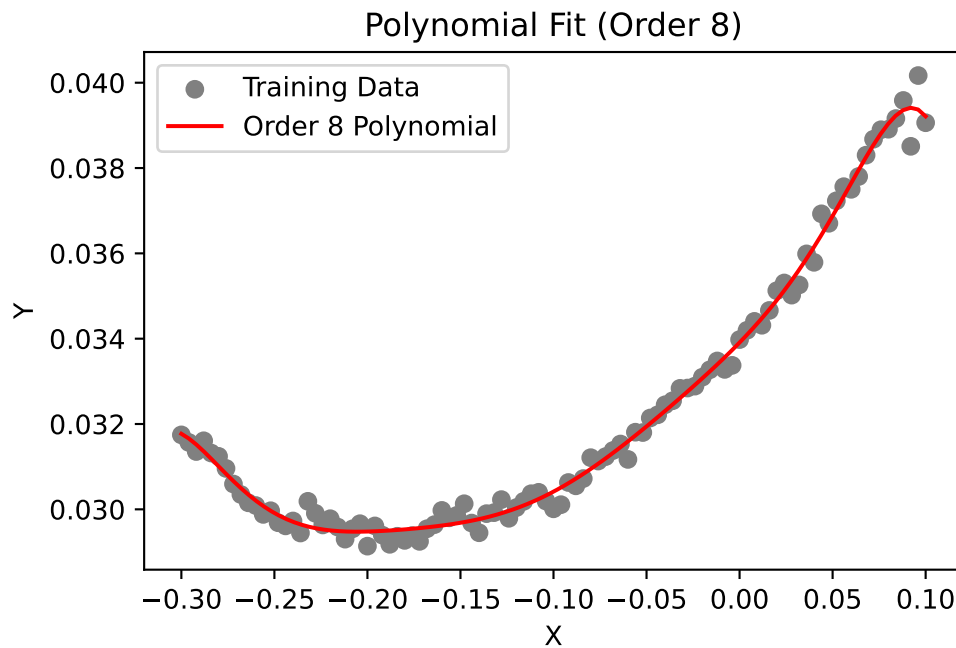
Figure 75.1.: Aerofoil drag data
