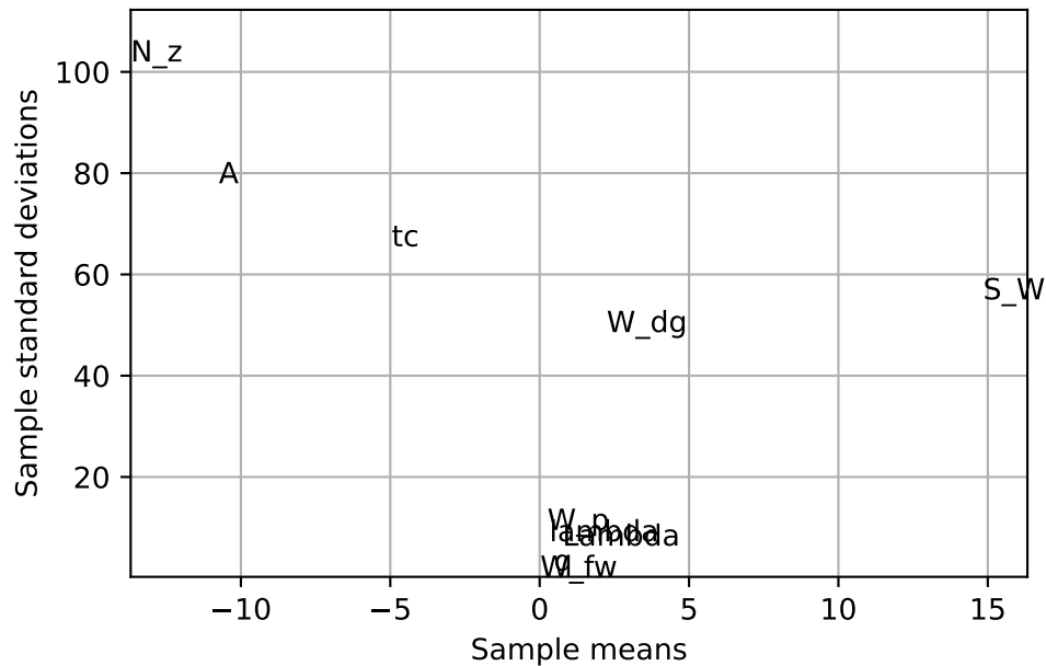
Figure 72.2.: Estimated means and standard deviations of the elementary effects for the 10 design variables of the wing weight function. Example based on Forrester, Sóbester, and Keane (2008).
