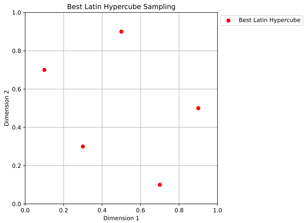
Figure 72.10.: Best Latin Hypercube Sampling
