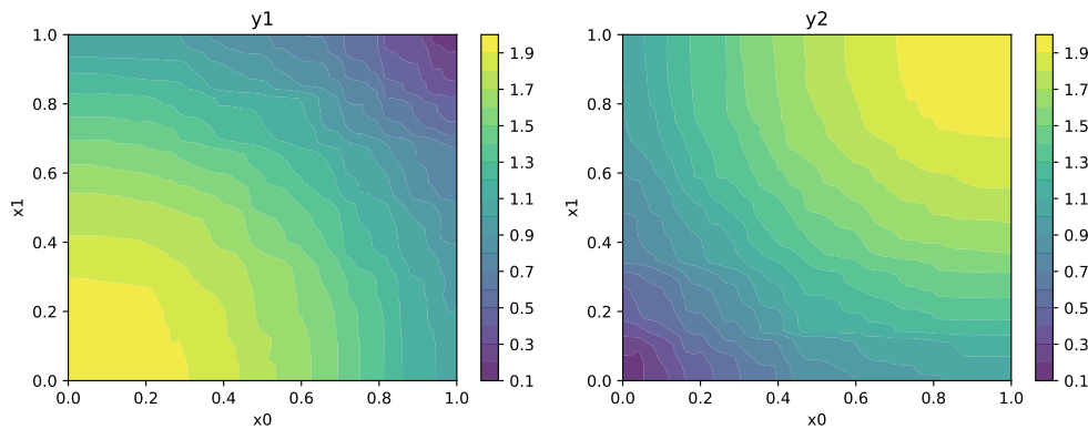
Figure 29.2.: Contours of the two objectives of the mo_conv2_max function
