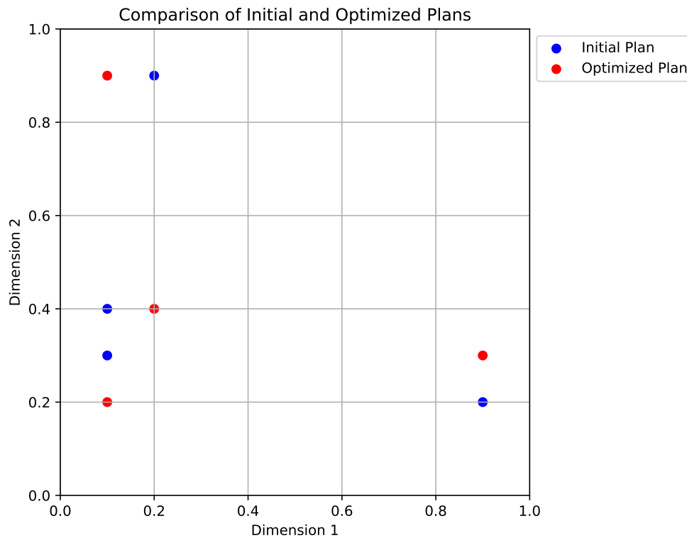
Figure 72.9.: Comparison of the initial and optimized plans in 2D.
