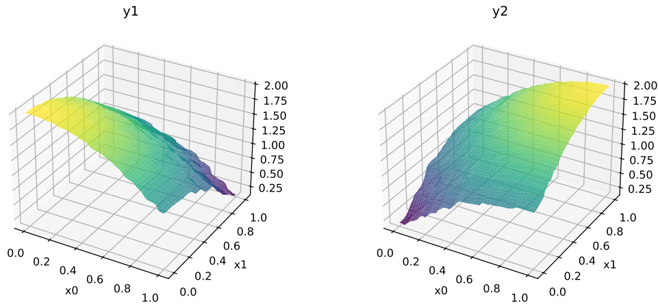
Figure 29.1.: Surfaces of the two objectives of the mo_conv2_max function
