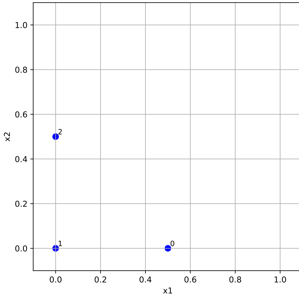
Figure 72.1.: Random orientation of the sampling matrix in 2-D. The labels indicate the row index of the points.
