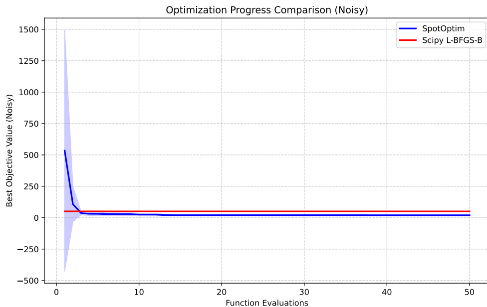
Figure 80.2.: Convergence Plot: Mean Best-So-Far Objective Value (Noisy) vs. Evaluations
