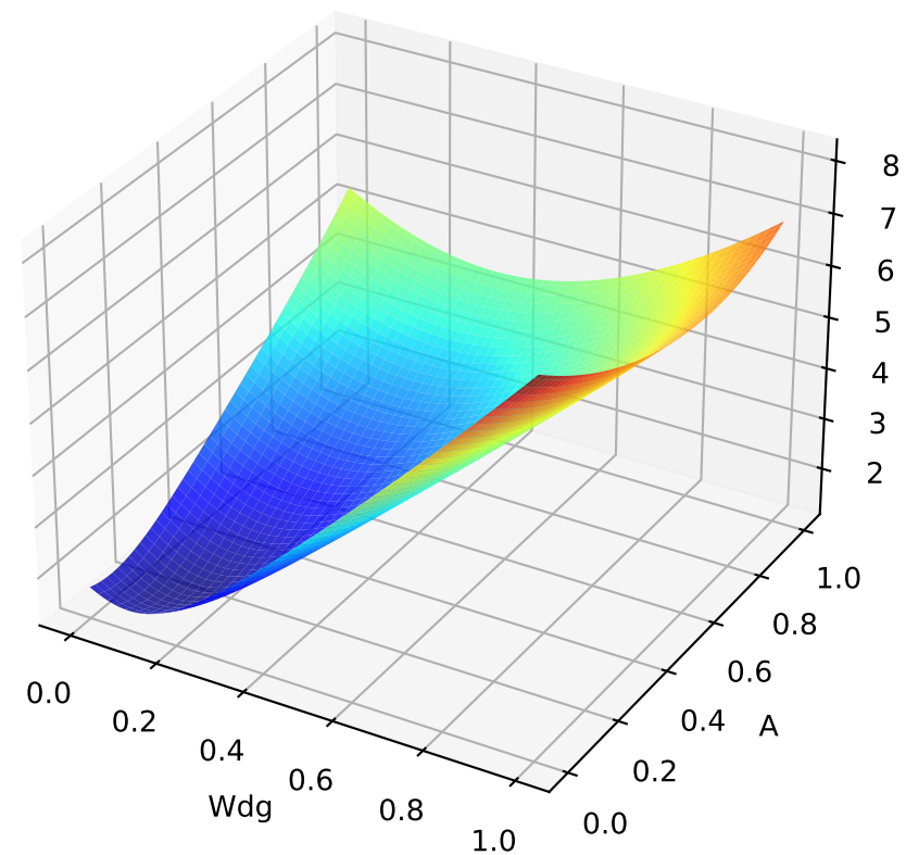
Uncertainty Contour
