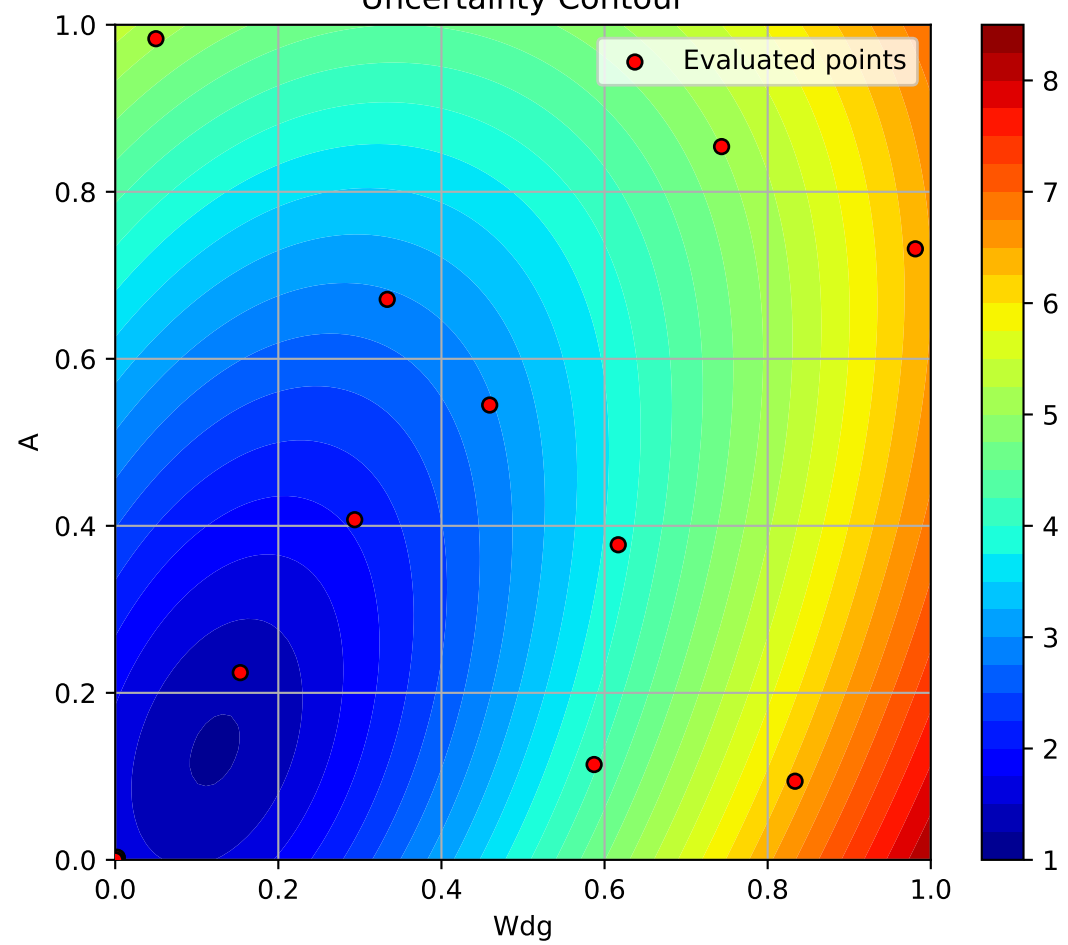
Uncertainty Contour
