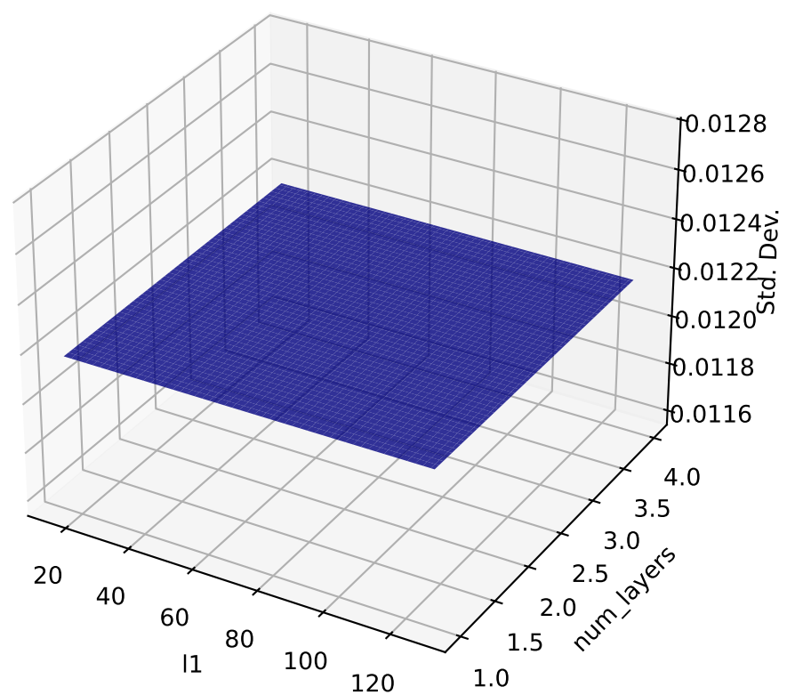
Uncertainty Contour
