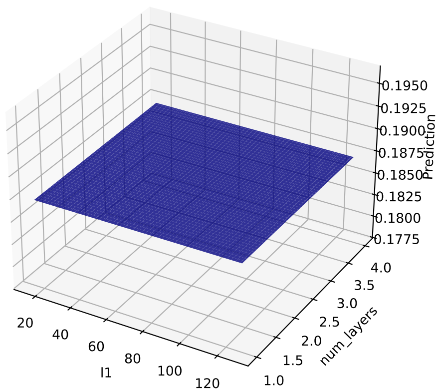
Prediction Contour
