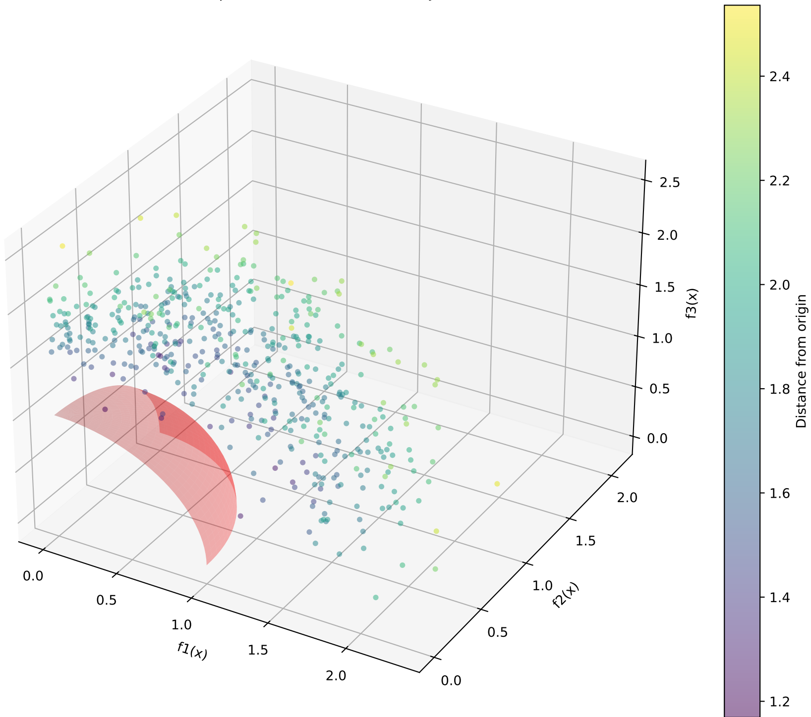
DTLZ2: Spherical Pareto Front (3 objectives)
