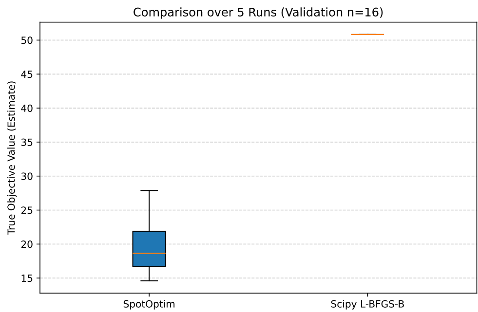
Figure 80.3.: Comparison of Validated True Means (Lower is Better)
