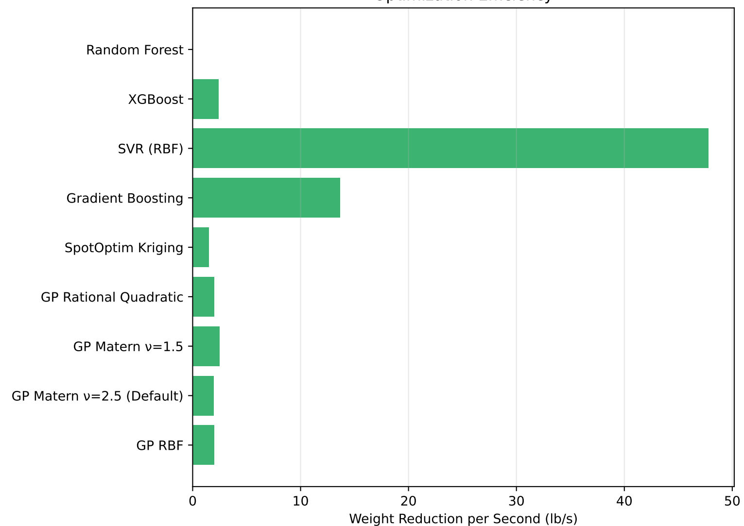
Optimization Efficiency
