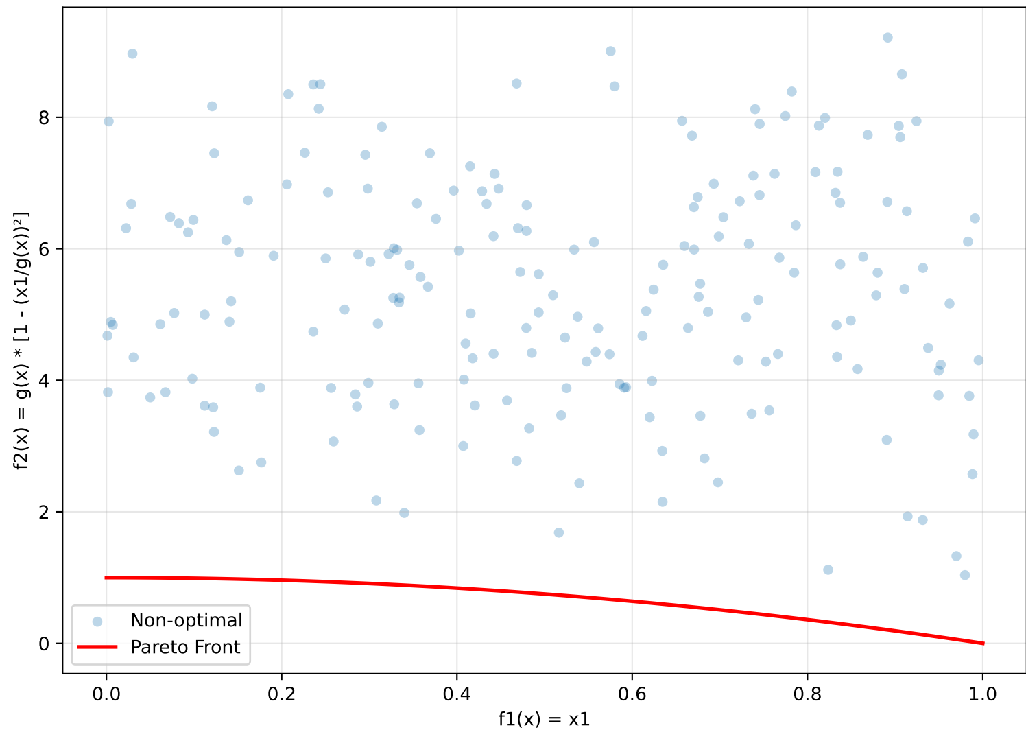
ZDT2: Non-Convex Pareto Front
