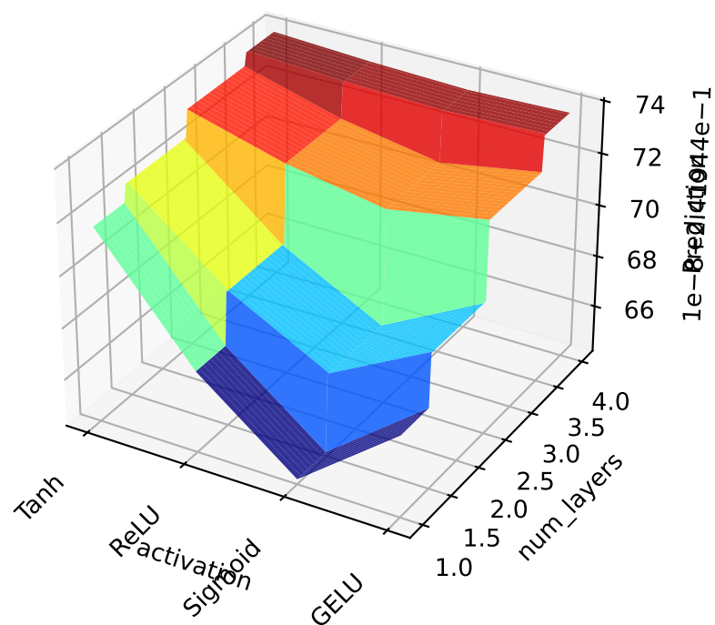
Prediction Contour
