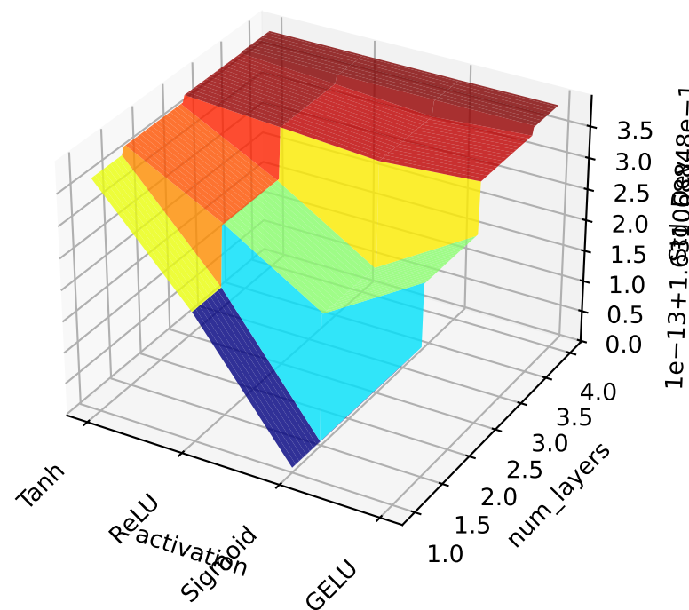
Uncertainty Contour
