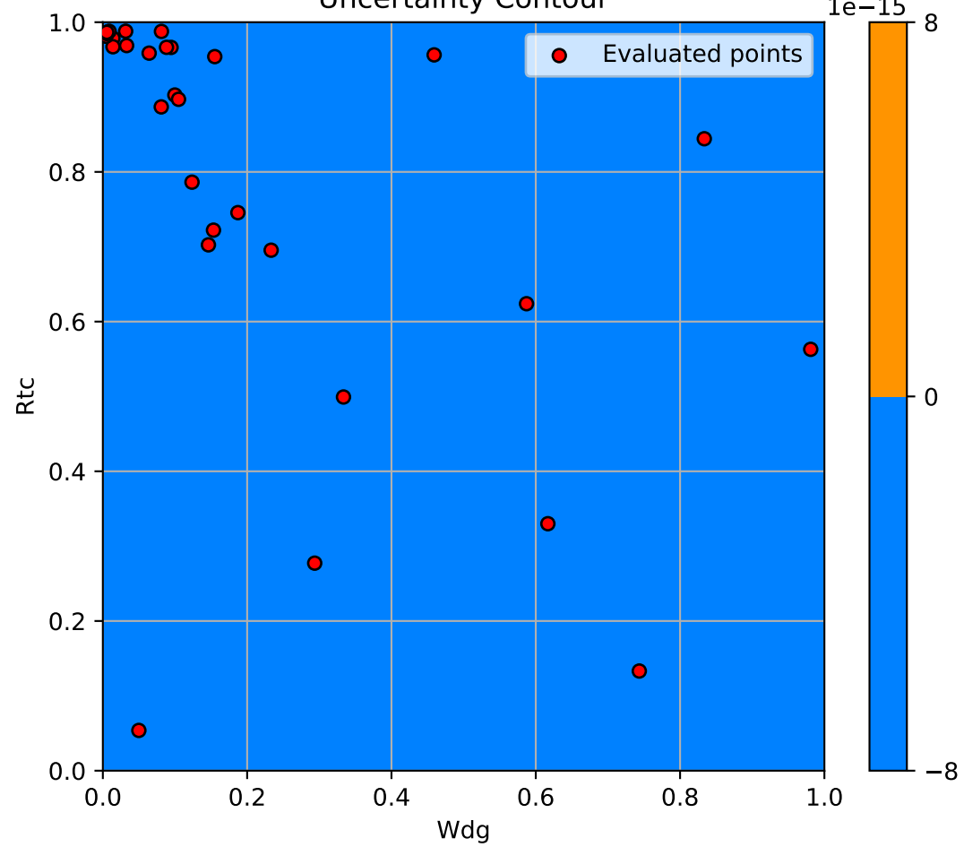
Uncertainty Contour
