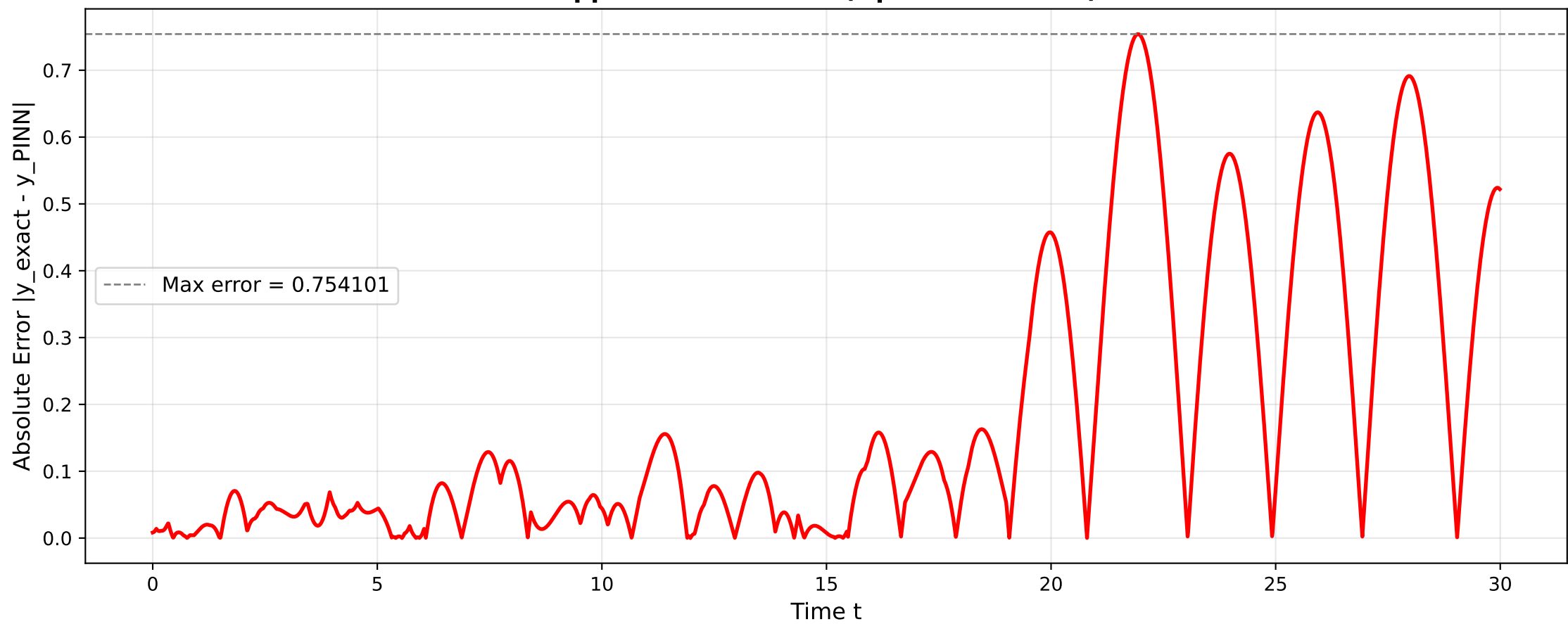
Approximation Error (Optimized Model)
