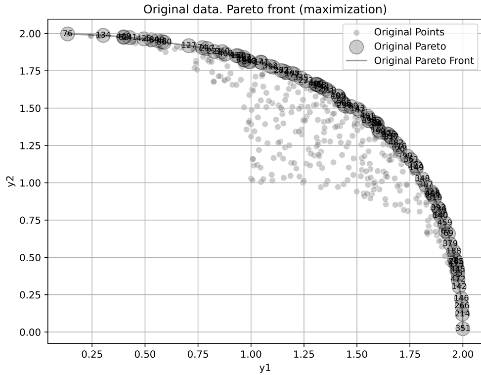
Figure 50.3.: Pareto front of the original data
