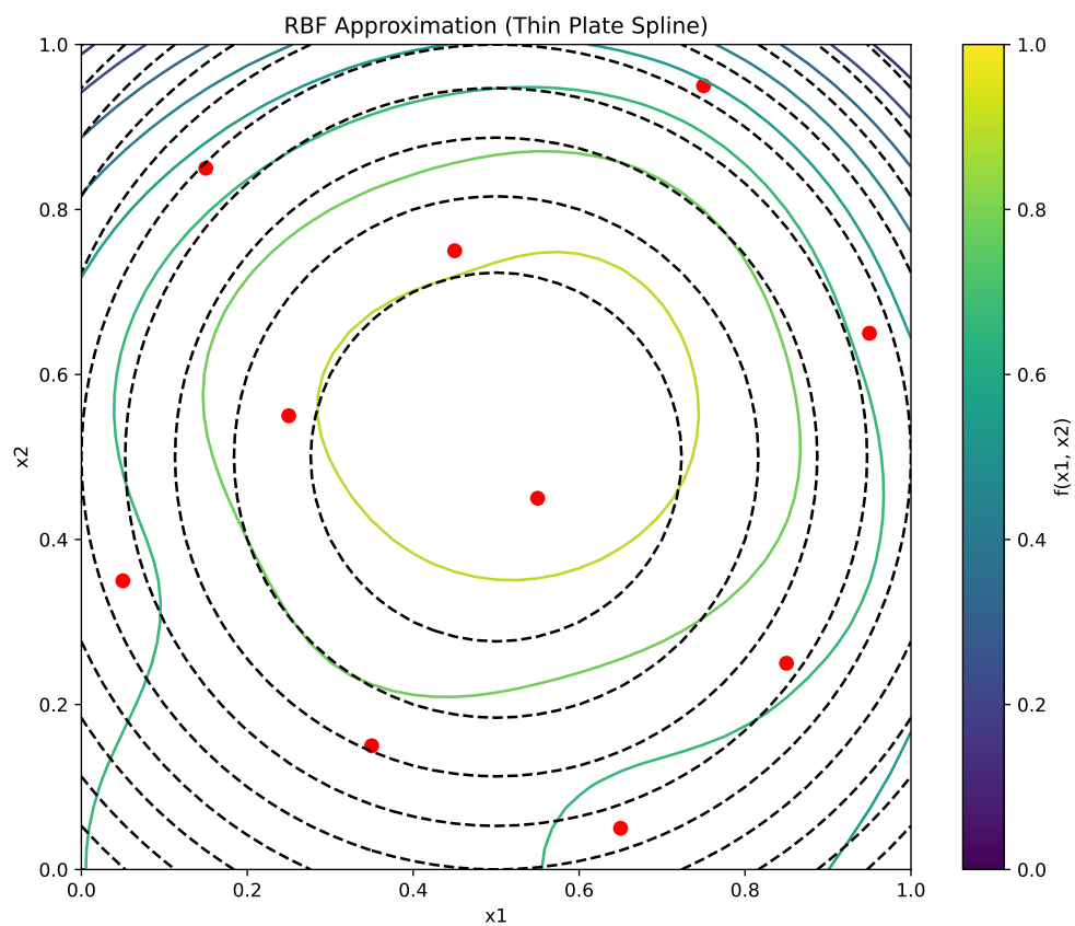
Figure 70.3.: RBF Approximation.
