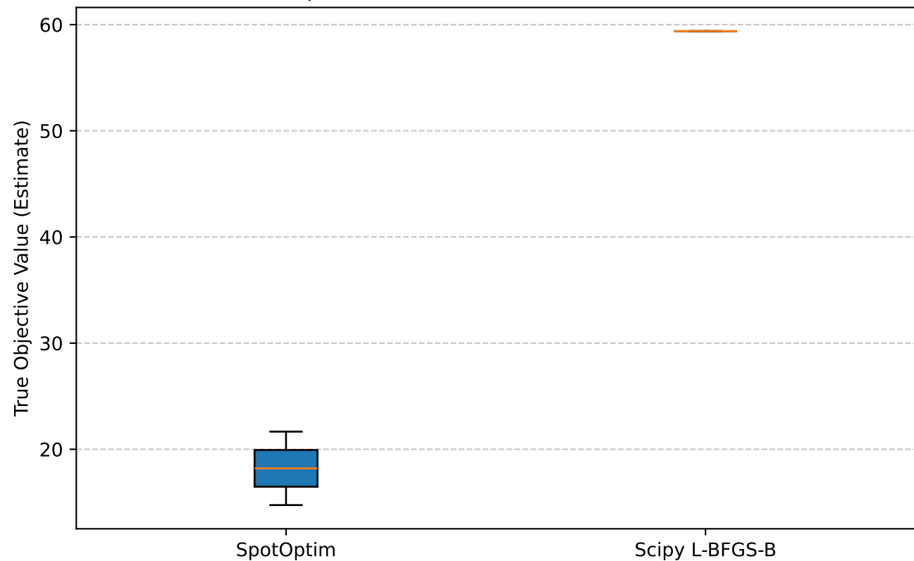
Comparison over 2 Runs (Validation n=16)
