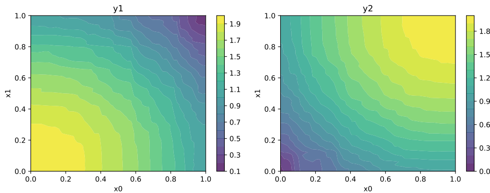
Figure 50.2.: Contours of the two objectives of the mo_conv2_max function
