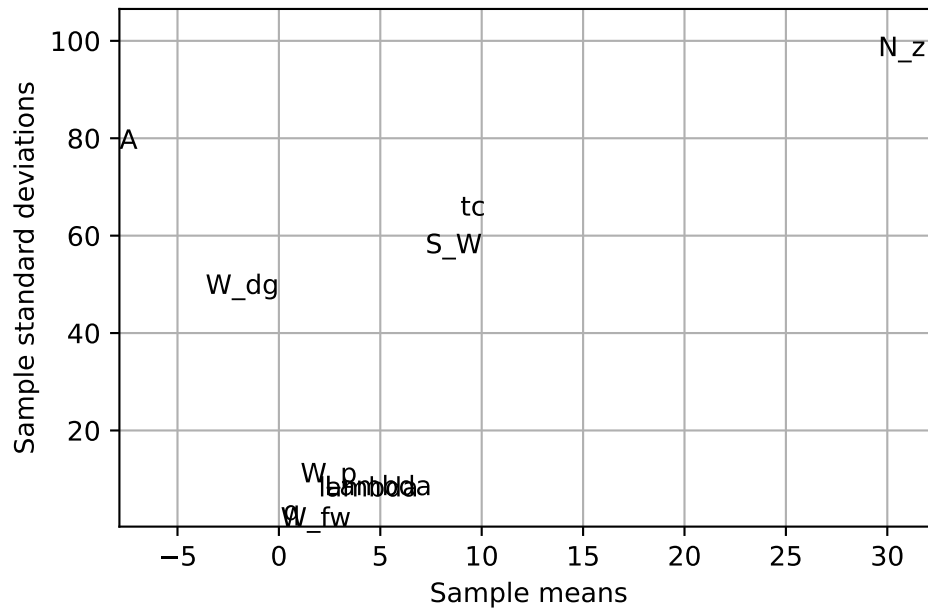
Figure 3.2.: Estimated means and standard deviations of the elementary effects for the 10 design variables of the wing weight function. Example based on Forrester, Sóbester, and Keane (2008).
