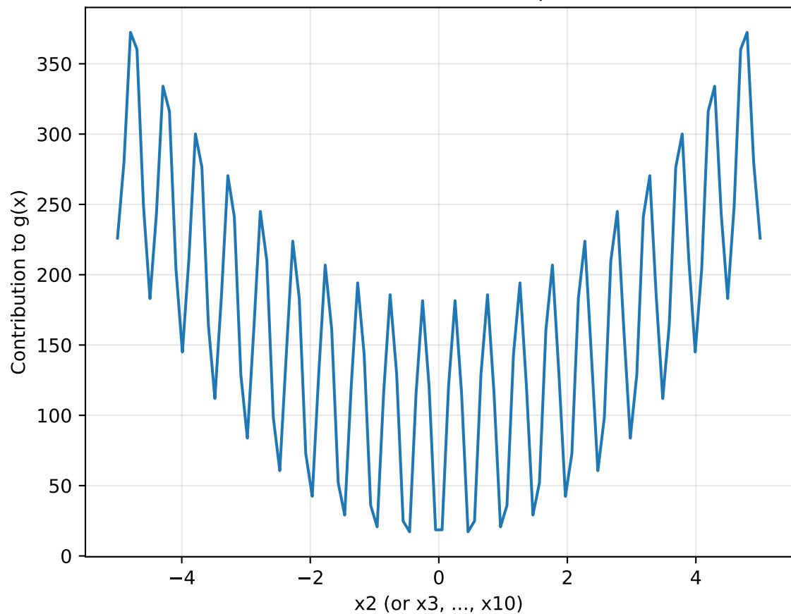
Multimodal Landscape
