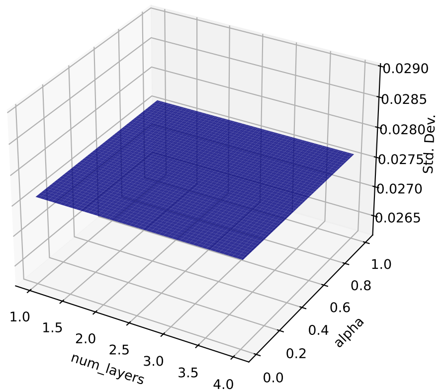
Uncertainty Contour
