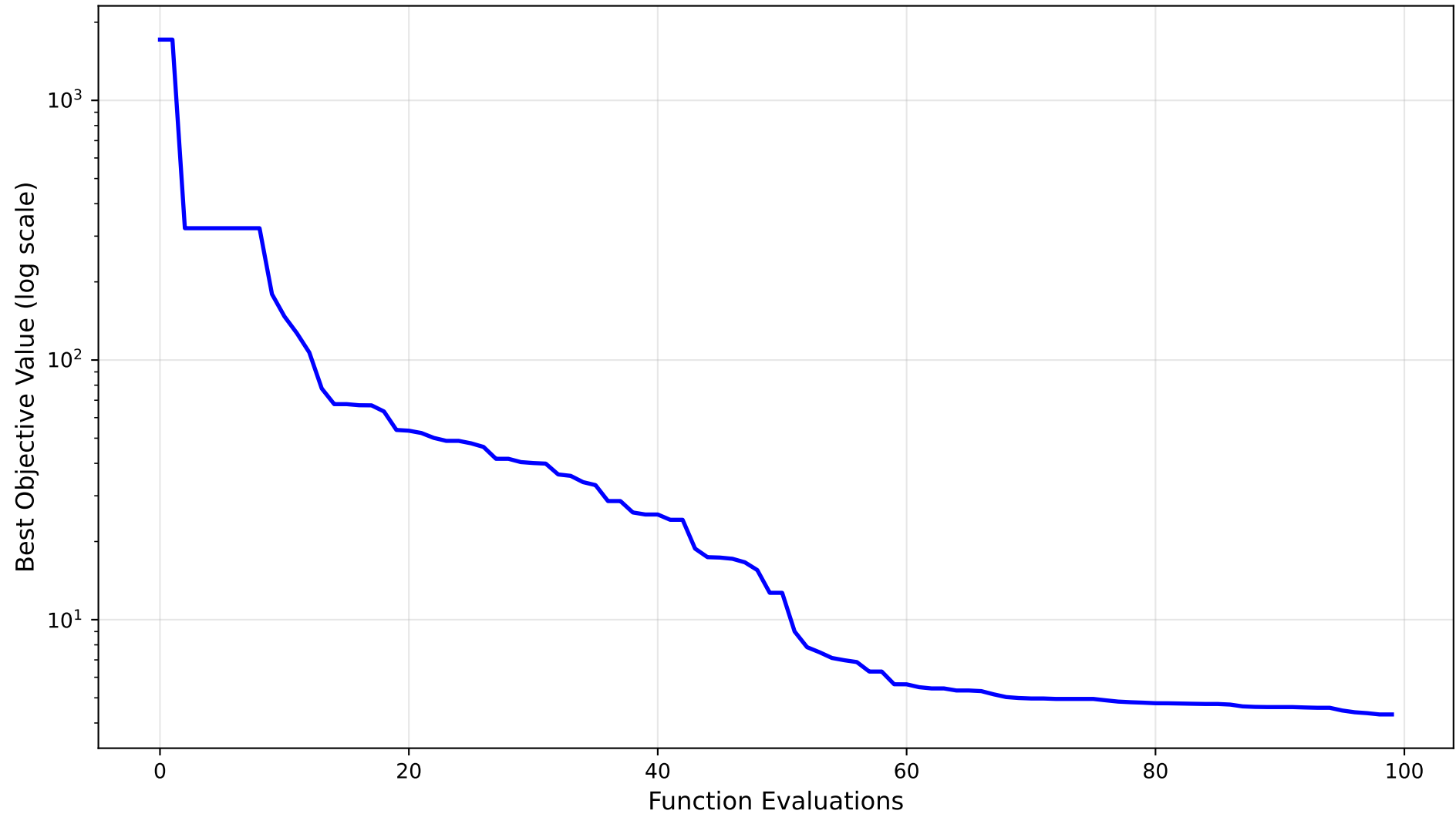
6D Rosenbrock: Sklearn Kriging Progress
