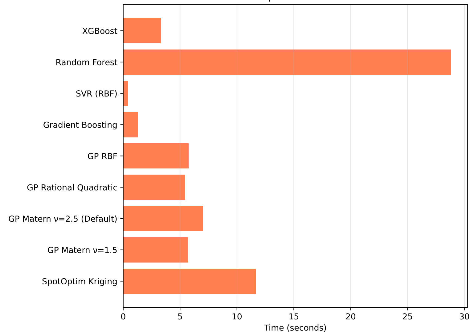
Optimization Efficiency
