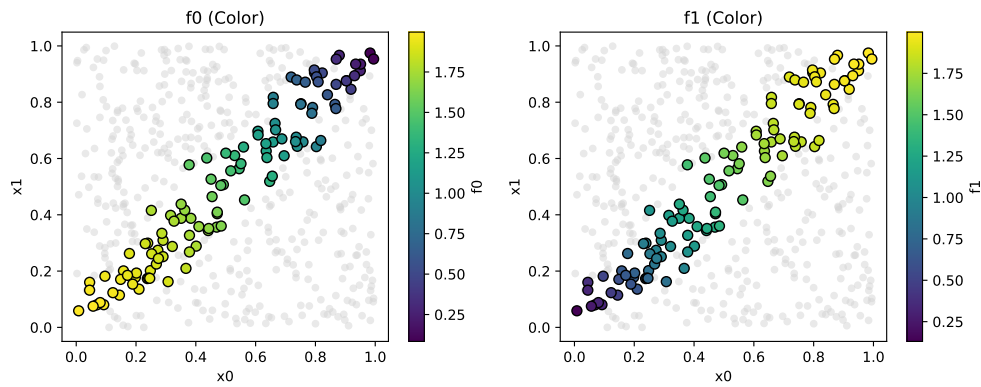
Figure 51.4.: Pareto-optimal points in the input space
