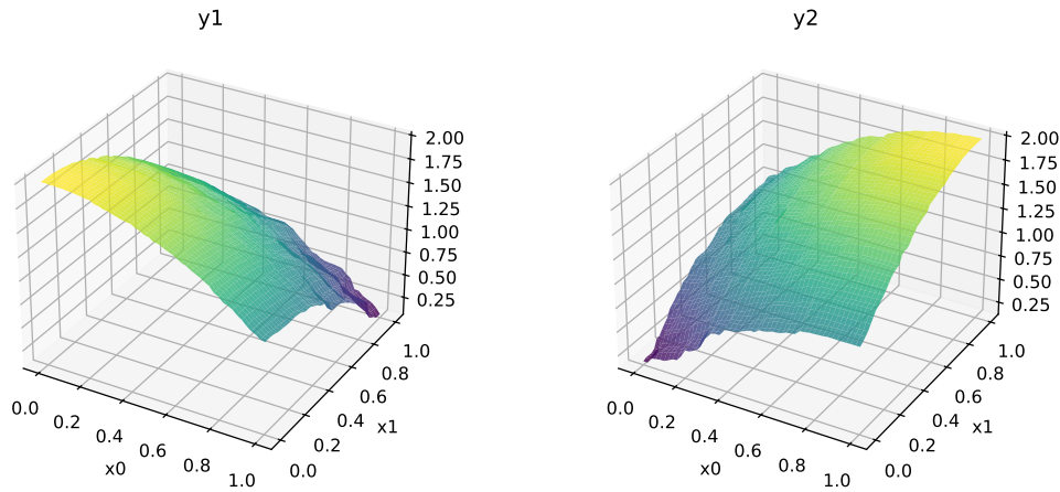
Figure 51.1.: Surfaces of the two objectives of the mo_conv2_max function
