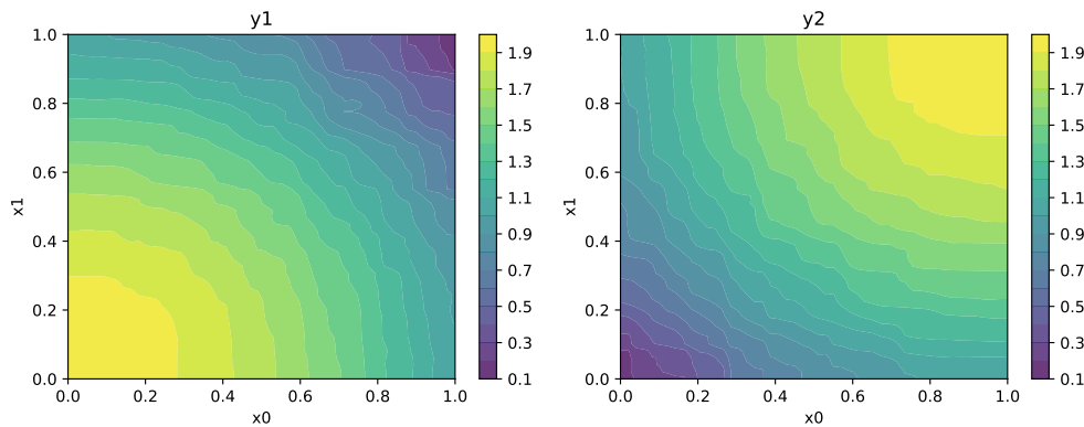
Figure 51.2.: Contours of the two objectives of the mo_conv2_max function
