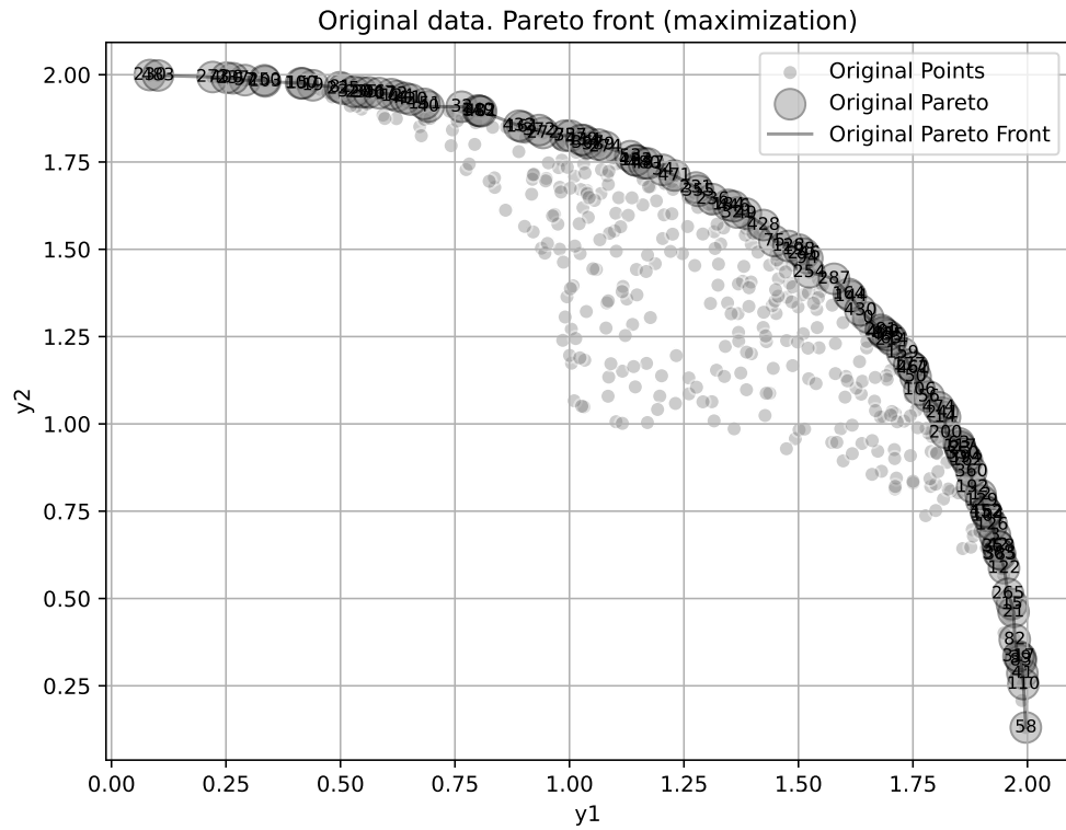
Figure 51.3.: Pareto front of the original data
