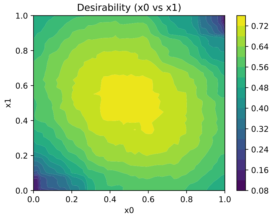
Figure 51.5.: Desirability function for multi-objective optimization
