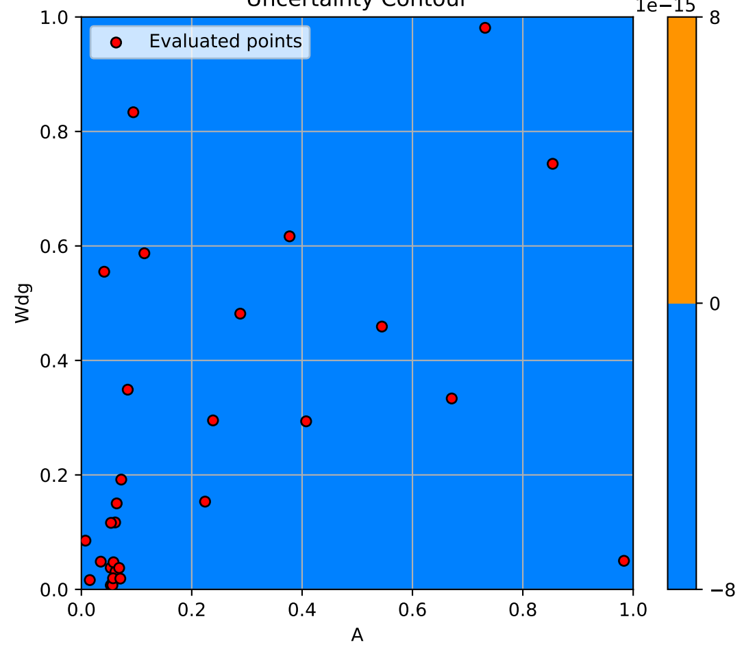
Uncertainty Contour
