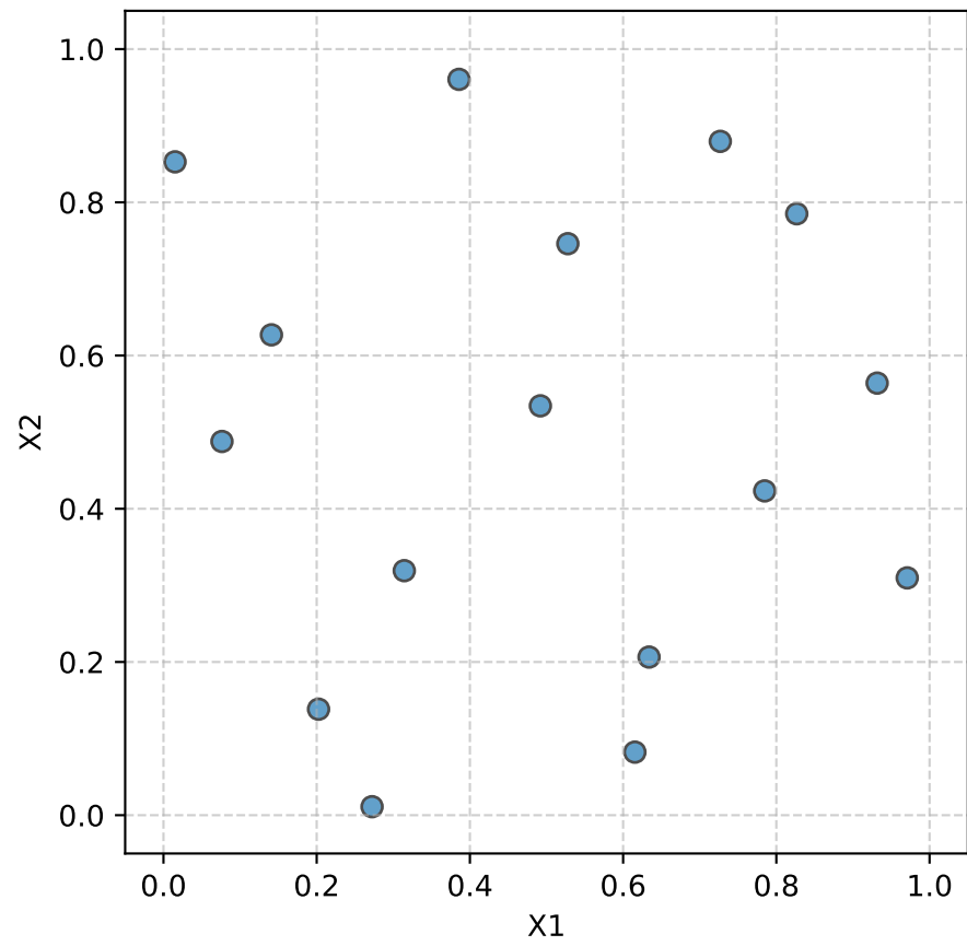
Random mmphi = 48.933
