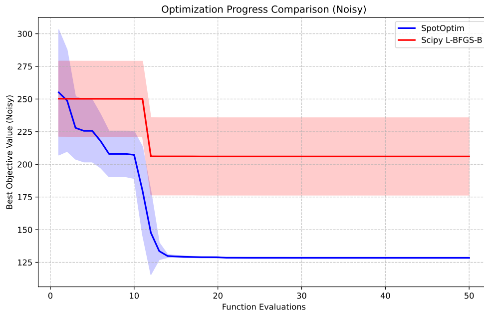
Figure 11.1.: Convergence Plot: Mean Best-So-Far Objective Value (Noisy) vs. Evaluations
