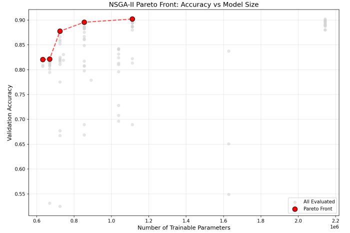
Fig. 2. NSGA-II: Pareto Front Plot
