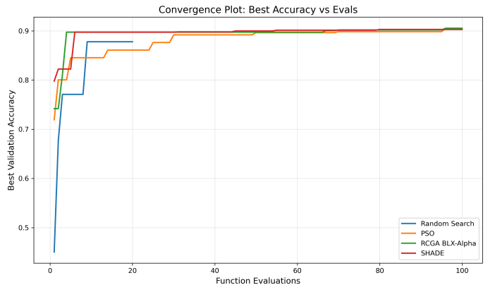
Fig. 1. Best Accuracy of Algorithm vs. Objective Evaluations
