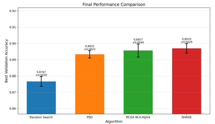
Fig. 3. Comparison of Final Performances on Three Seeds
