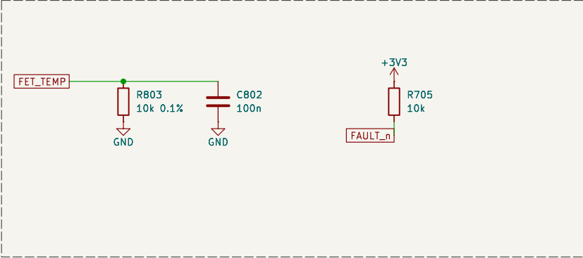
ADC3 divider, FAULT_n pull-up
