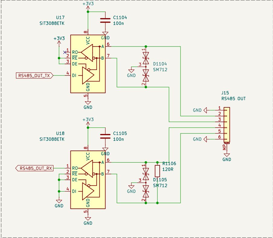
RS-485 relay: port OUT
