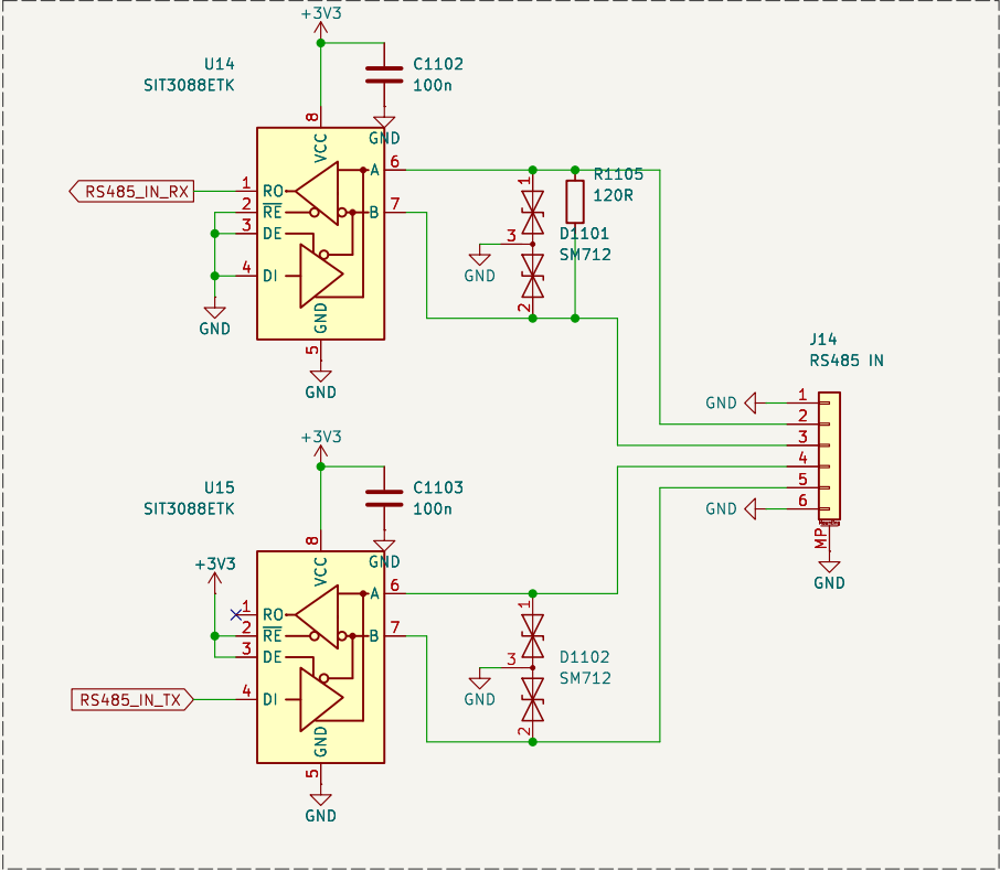
RS-485 relay: port IN
