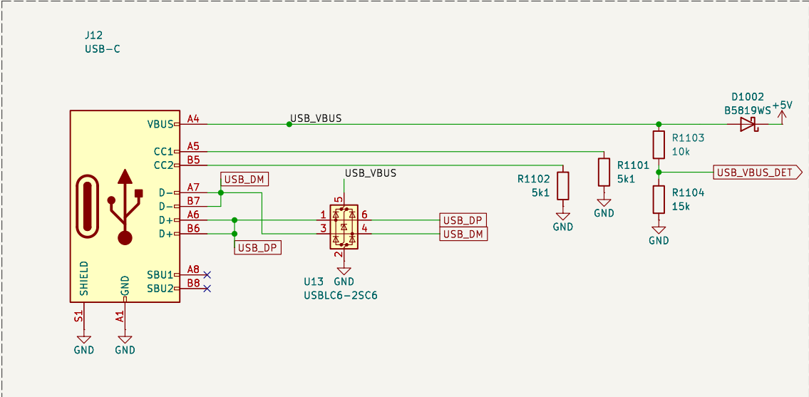
USB-C: data and 5 V logic, no PD
