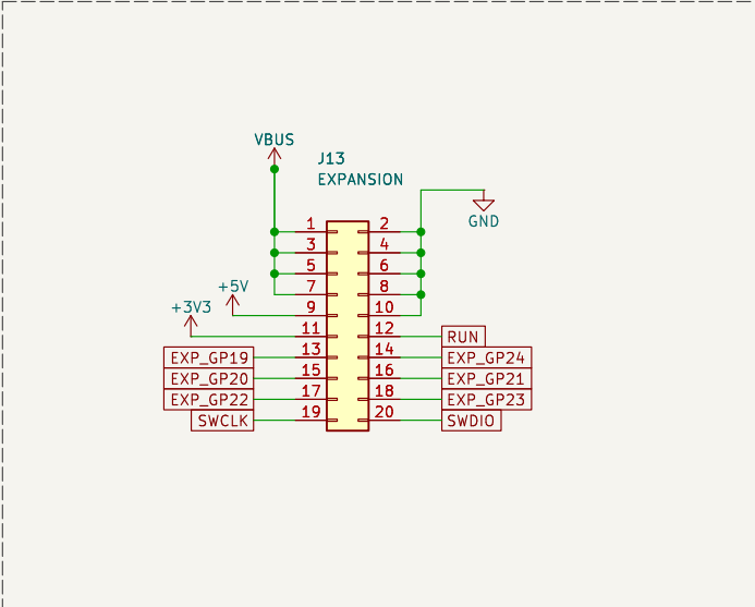
Expansion header: PD or Ethernet board
