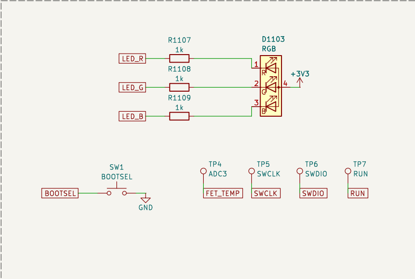
Status LED, BOOTSEL, test pads
