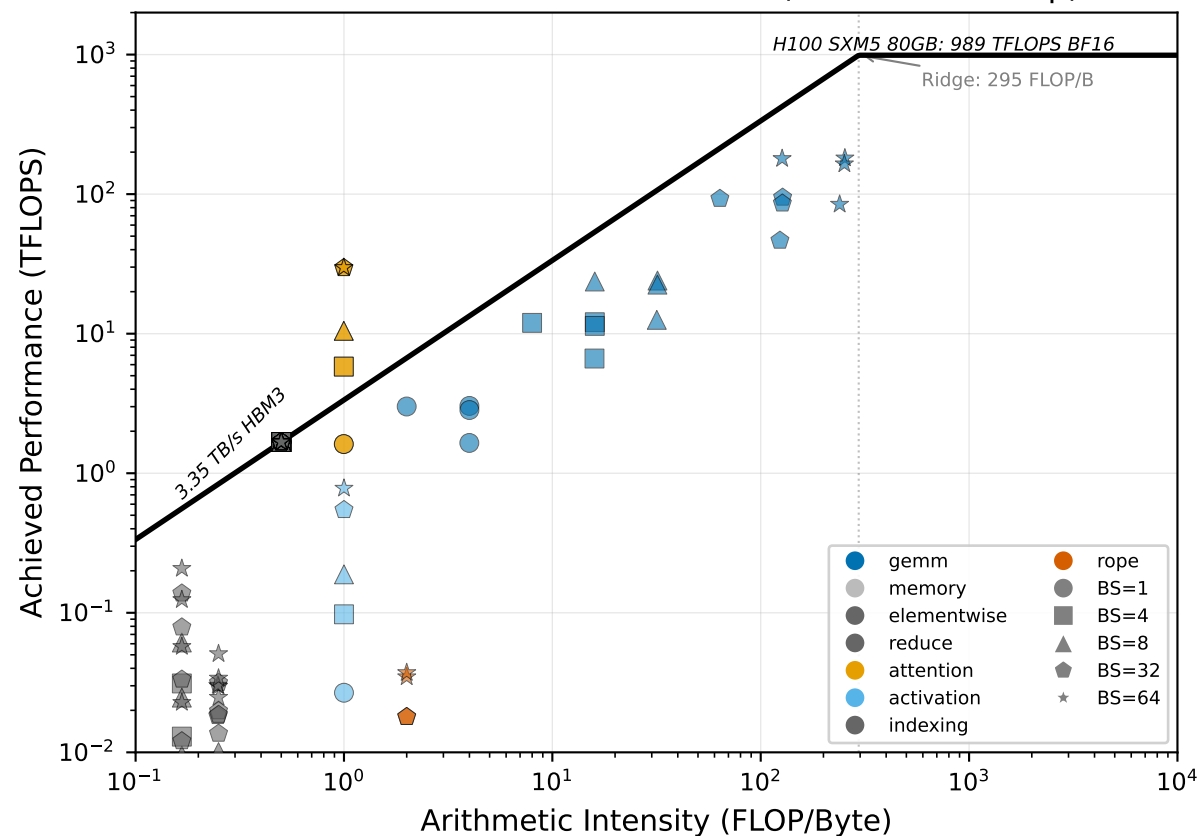
Llama-3.1-70B-Instruct — decode (batch size sweep)
