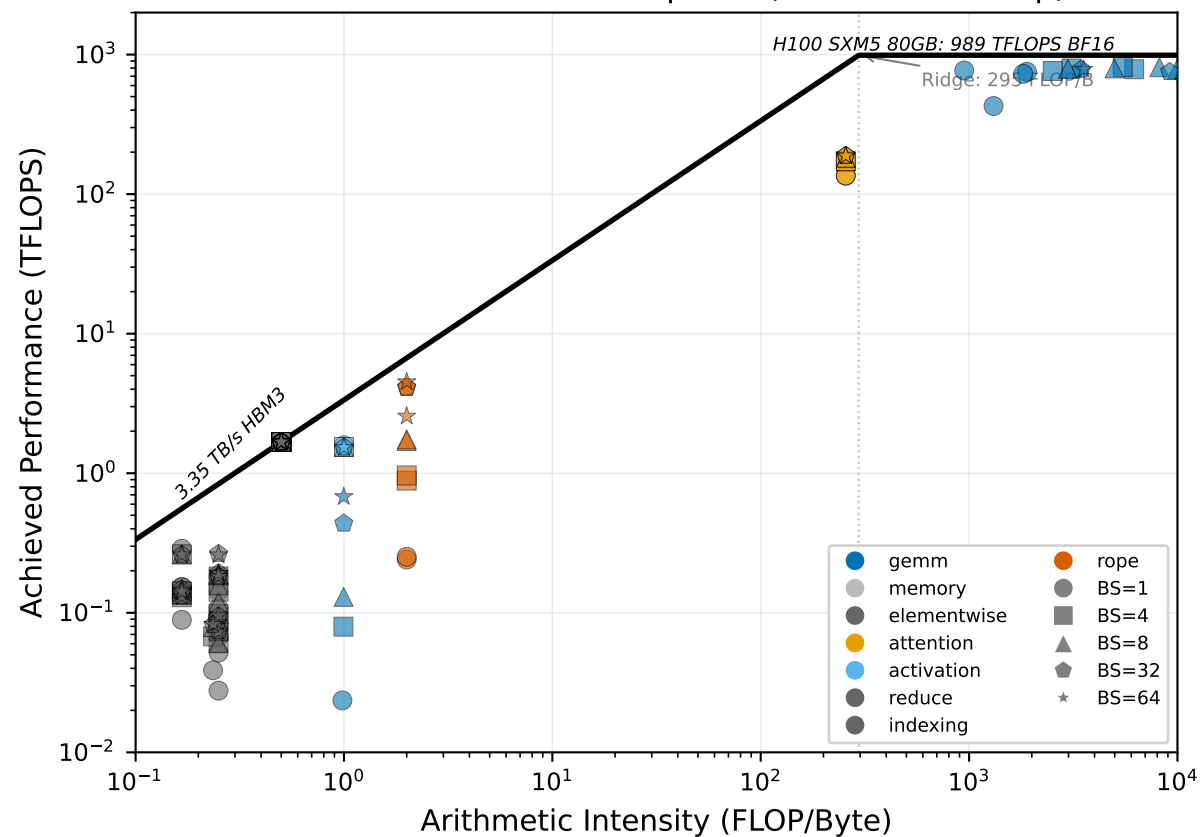
Llama-3.1-70B-Instruct — prefill (batch size sweep)
