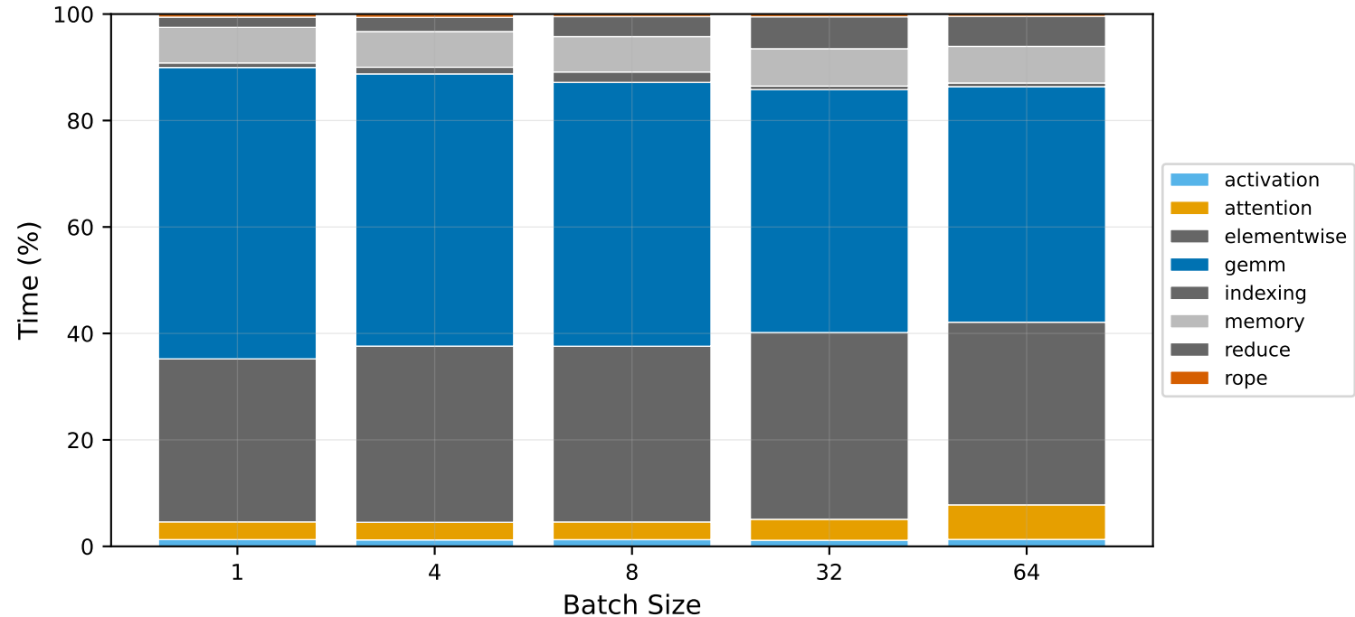
Llama-3.1-8B-Instruct — decode Kernel Time Breakdown
