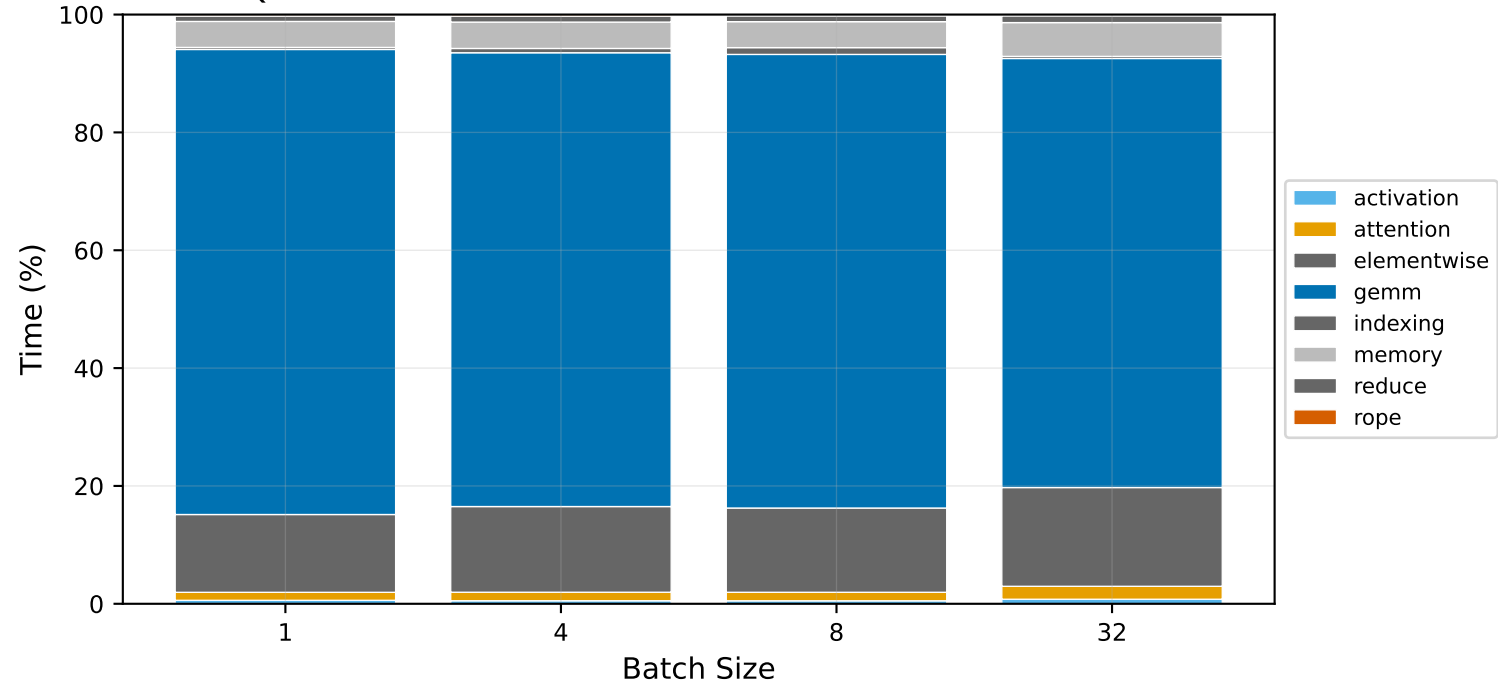
Qwen2.5-72B-Instruct — decode Kernel Time Breakdown
