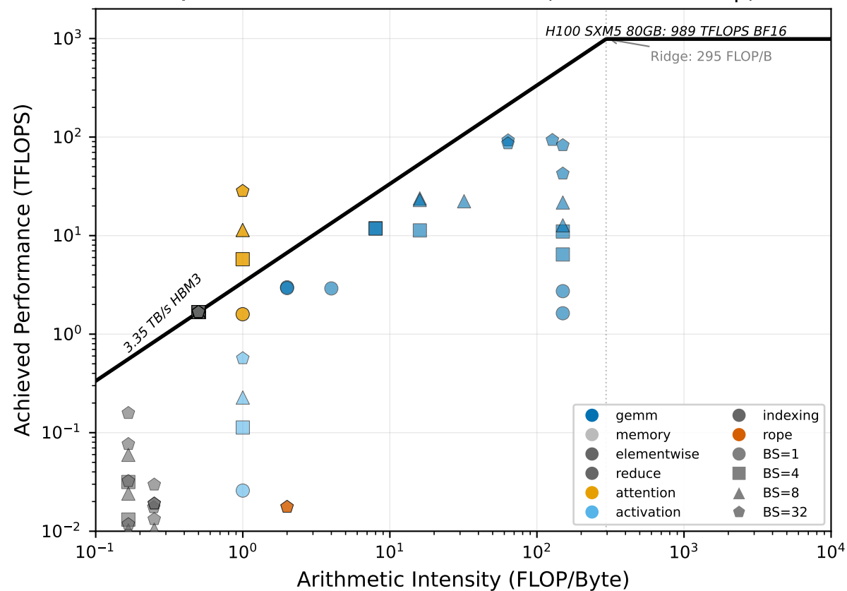
Qwen2.5-72B-Instruct — decode (batch size sweep)
