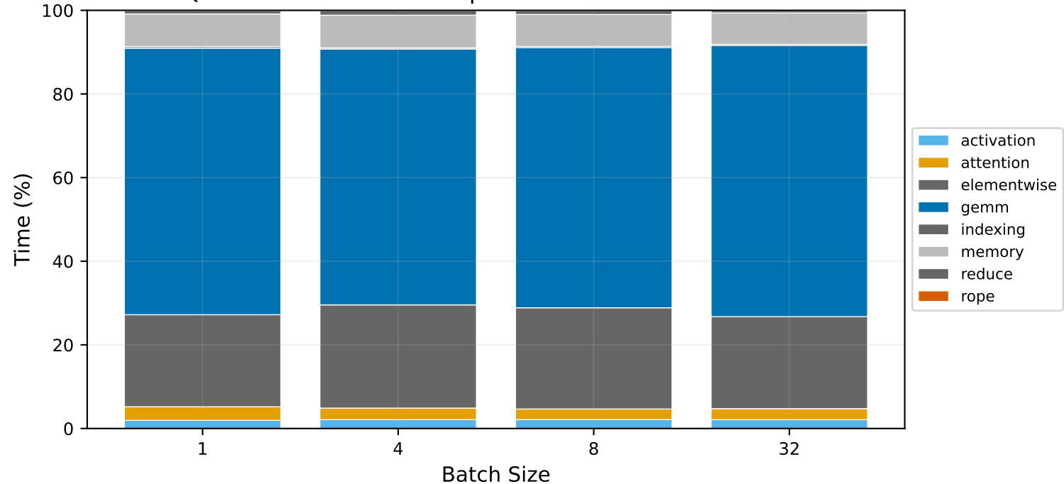
Qwen2.5-72B-Instruct — prefill Kernel Time Breakdown
