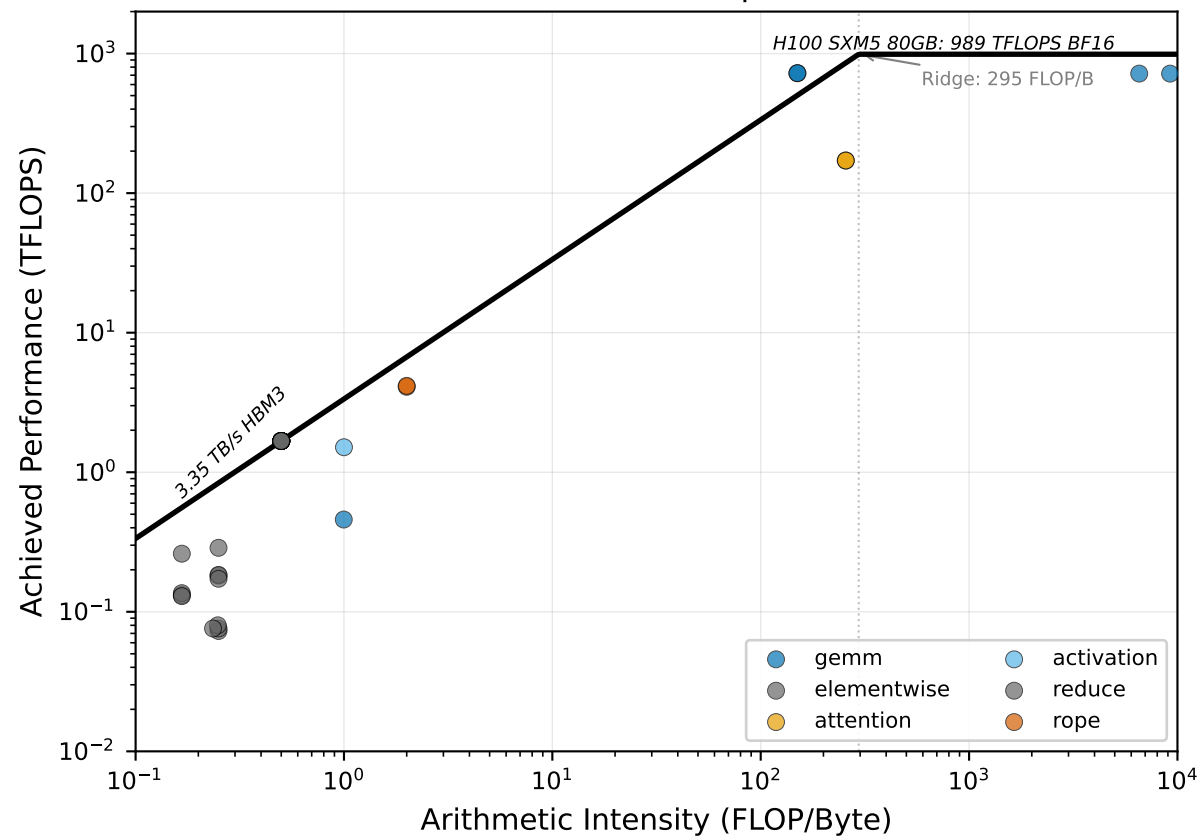
Qwen2.5-72B-Instruct — prefill (BS=32)
