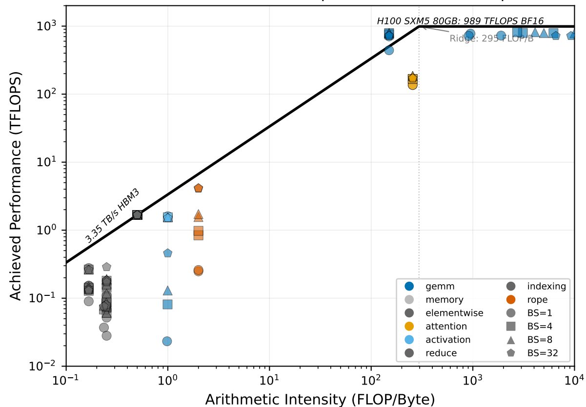
Qwen2.5-72B-Instruct — prefill (batch size sweep)
